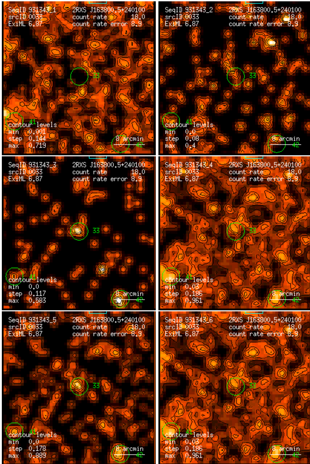
Figure 33: RASS 931343: detection 0033: band rate images, Gaussian filter: (1) PSPC channels 11 – 41, (2) 52 – 90, (3) 91 – 201, (4) 11 – 235, (5) 52 – 201, (6) 11 – 201. Broad band rates in counts/ks. Band rate contour levels in counts/ks/arcmin 2 .
