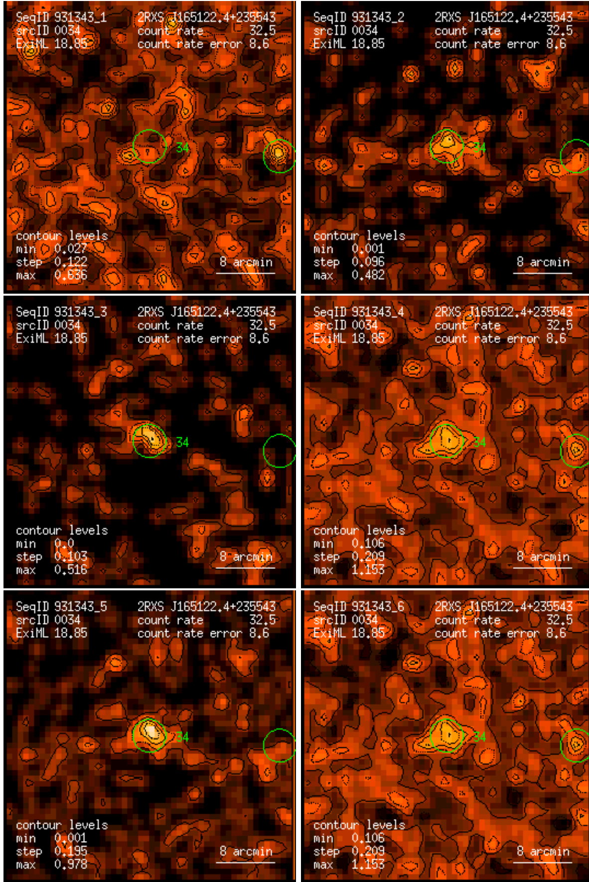
Figure 34: RASS 931343: detection 0034: band rate images, Gaussian filter: (1) PSPC channels 11 – 41, (2) 52 – 90, (3) 91 – 201, (4) 11 – 235, (5) 52 – 201, (6) 11 – 201. Broad band rates in counts/ks. Band rate contour levels in counts/ks/arcmin 2 .
