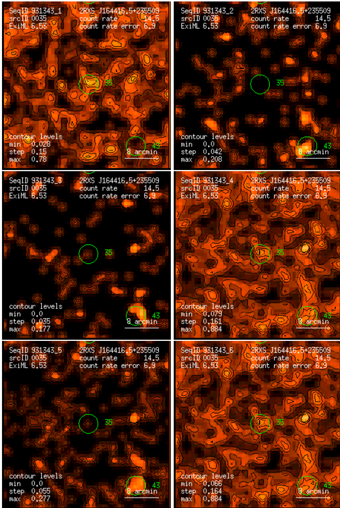
Figure 35: RASS 931343: detection 0035: band rate images, Gaussian filter: (1) PSPC channels 11 – 41, (2) 52 – 90, (3) 91 – 201, (4) 11 – 235, (5) 52 – 201, (6) 11 – 201. Broad band rates in counts/ks. Band rate contour levels in counts/ks/arcmin 2 .
