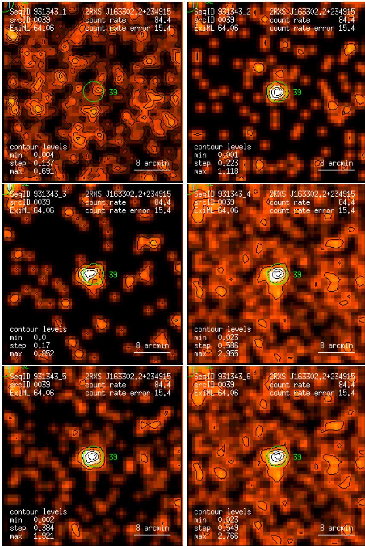
Figure 39: RASS 931343: detection 0039: band rate images, Gaussian filter: (1) PSPC channels 11 – 41, (2) 52 – 90, (3) 91 – 201, (4) 11 – 235, (5) 52 – 201, (6) 11 – 201. Broad band rates in counts/ks. Band rate contour levels in counts/ks/arcmin 2 .
