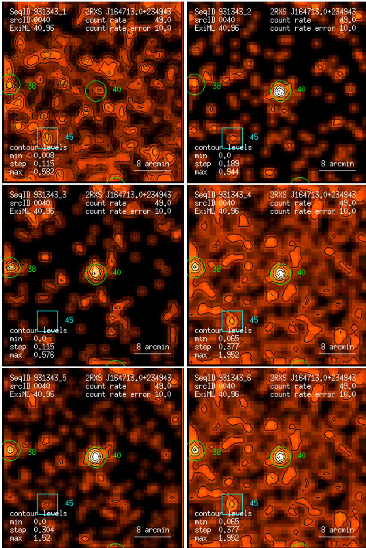
Figure 40: RASS 931343: detection 0040: band rate images, Gaussian filter: (1) PSPC channels 11 – 41, (2) 52 – 90, (3) 91 – 201, (4) 11 – 235, (5) 52 – 201, (6) 11 – 201. Broad band rates in counts/ks. Band rate contour levels in counts/ks/arcmin 2 .
