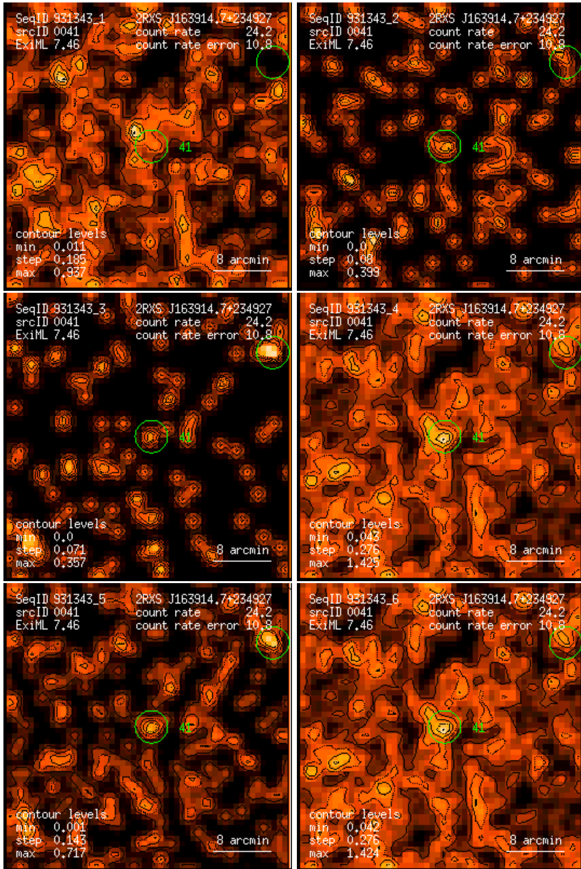
Figure 41: RASS 931343: detection 0041: band rate images, Gaussian filter: (1) PSPC channels 11 – 41, (2) 52 – 90, (3) 91 – 201, (4) 11 – 235, (5) 52 – 201, (6) 11 – 201. Broad band rates in counts/ks. Band rate contour levels in counts/ks/arcmin 2 .
