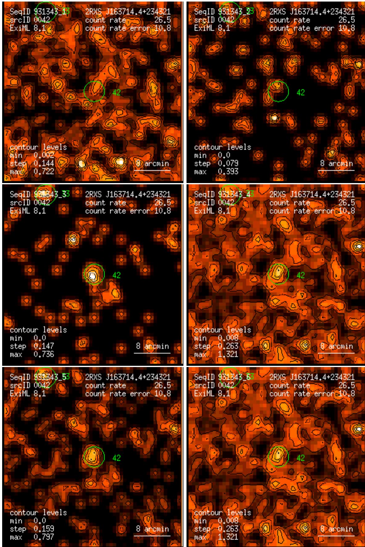
Figure 42: RASS 931343: detection 0042: band rate images, Gaussian filter: (1) PSPC channels 11 – 41, (2) 52 – 90, (3) 91 – 201, (4) 11 – 235, (5) 52 – 201, (6) 11 – 201. Broad band rates in counts/ks. Band rate contour levels in counts/ks/arcmin 2 .
