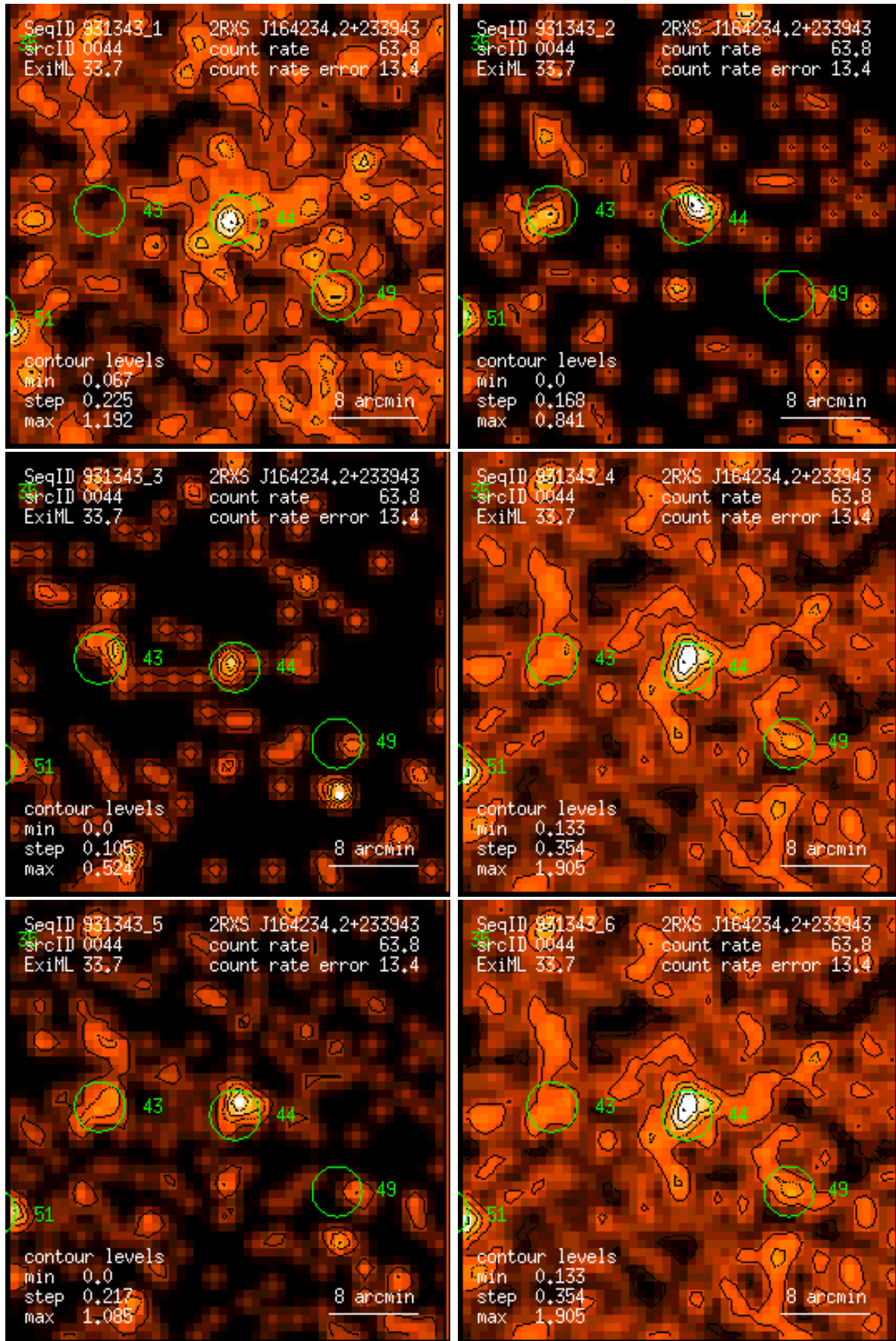
Figure 44: RASS 931343: detection 0044: band rate images, Gaussian filter: (1) PSPC channels 11 – 41, (2) 52 – 90, (3) 91 – 201, (4) 11 – 235, (5) 52 – 201, (6) 11 – 201. Broad band rates in counts/ks. Band rate contour levels in counts/ks/arcmin 2 .
