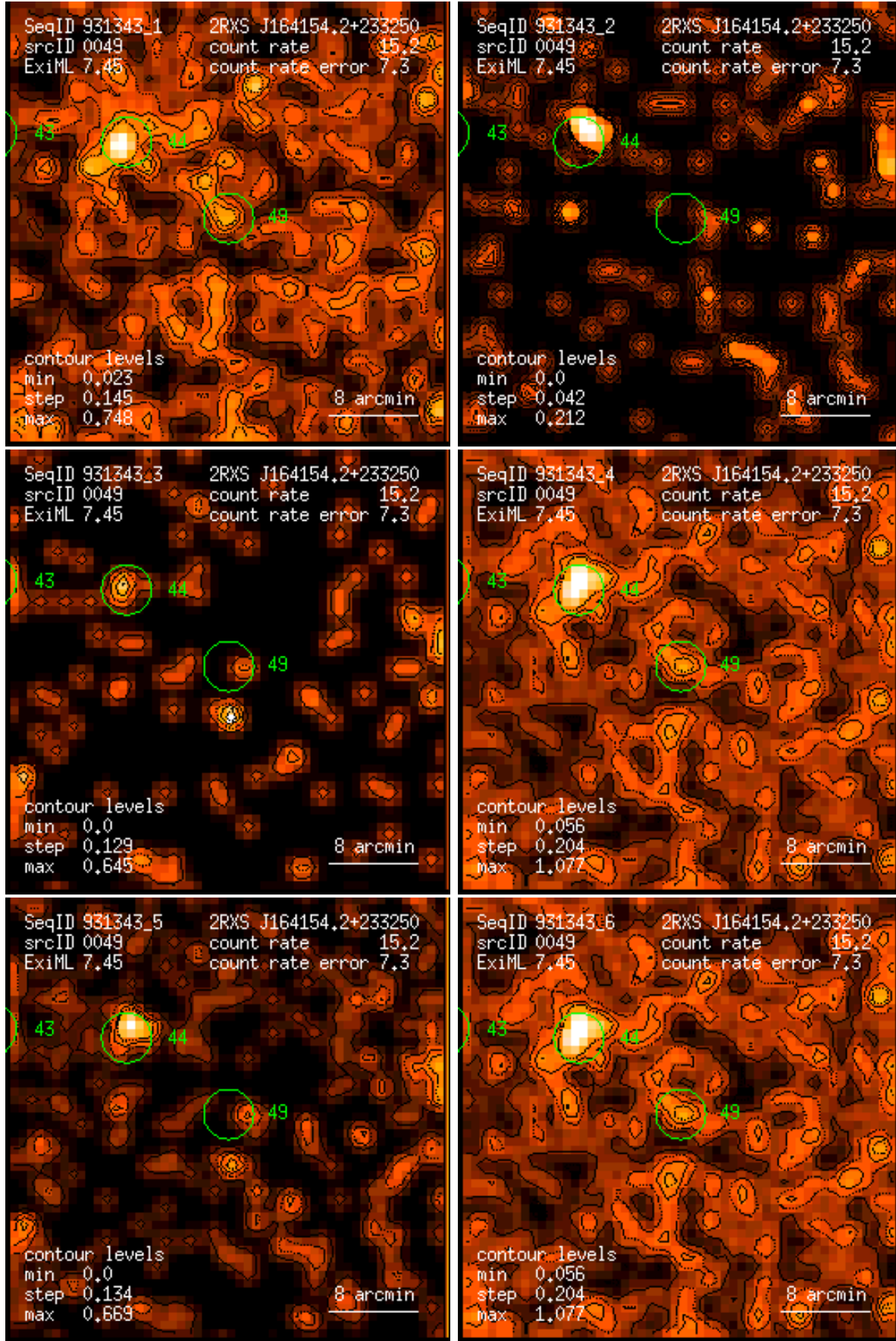
Figure 49: RASS 931343: detection 0049: band rate images, Gaussian filter: (1) PSPC channels 11 – 41, (2) 52 – 90, (3) 91 – 201, (4) 11 – 235, (5) 52 – 201, (6) 11 – 201. Broad band rates in counts/ks. Band rate contour levels in counts/ks/arcmin 2 .
