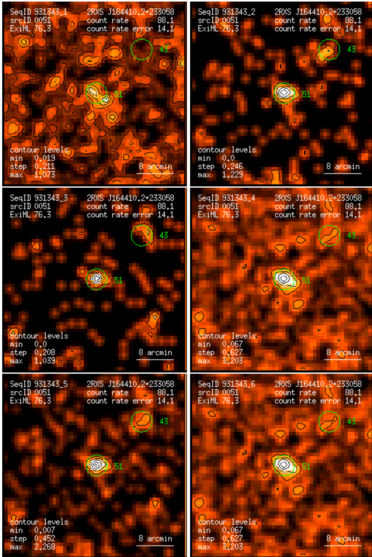
Figure 51: RASS 931343: detection 0051: band rate images, Gaussian filter: (1) PSPC channels 11 – 41, (2) 52 – 90, (3) 91 – 201, (4) 11 – 235, (5) 52 – 201, (6) 11 – 201. Broad band rates in counts/ks. Band rate contour levels in counts/ks/arcmin 2 .
