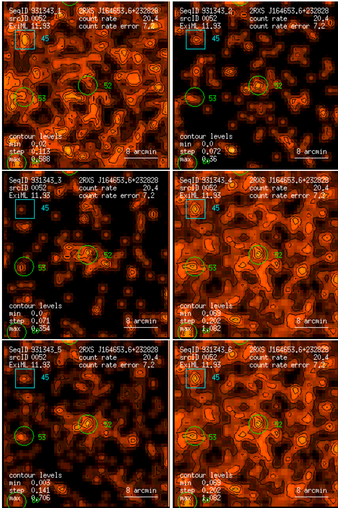
Figure 52: RASS 931343: detection 0052: band rate images, Gaussian filter: (1) PSPC channels 11 – 41, (2) 52 – 90, (3) 91 – 201, (4) 11 – 235, (5) 52 – 201, (6) 11 – 201. Broad band rates in counts/ks. Band rate contour levels in counts/ks/arcmin 2 .
