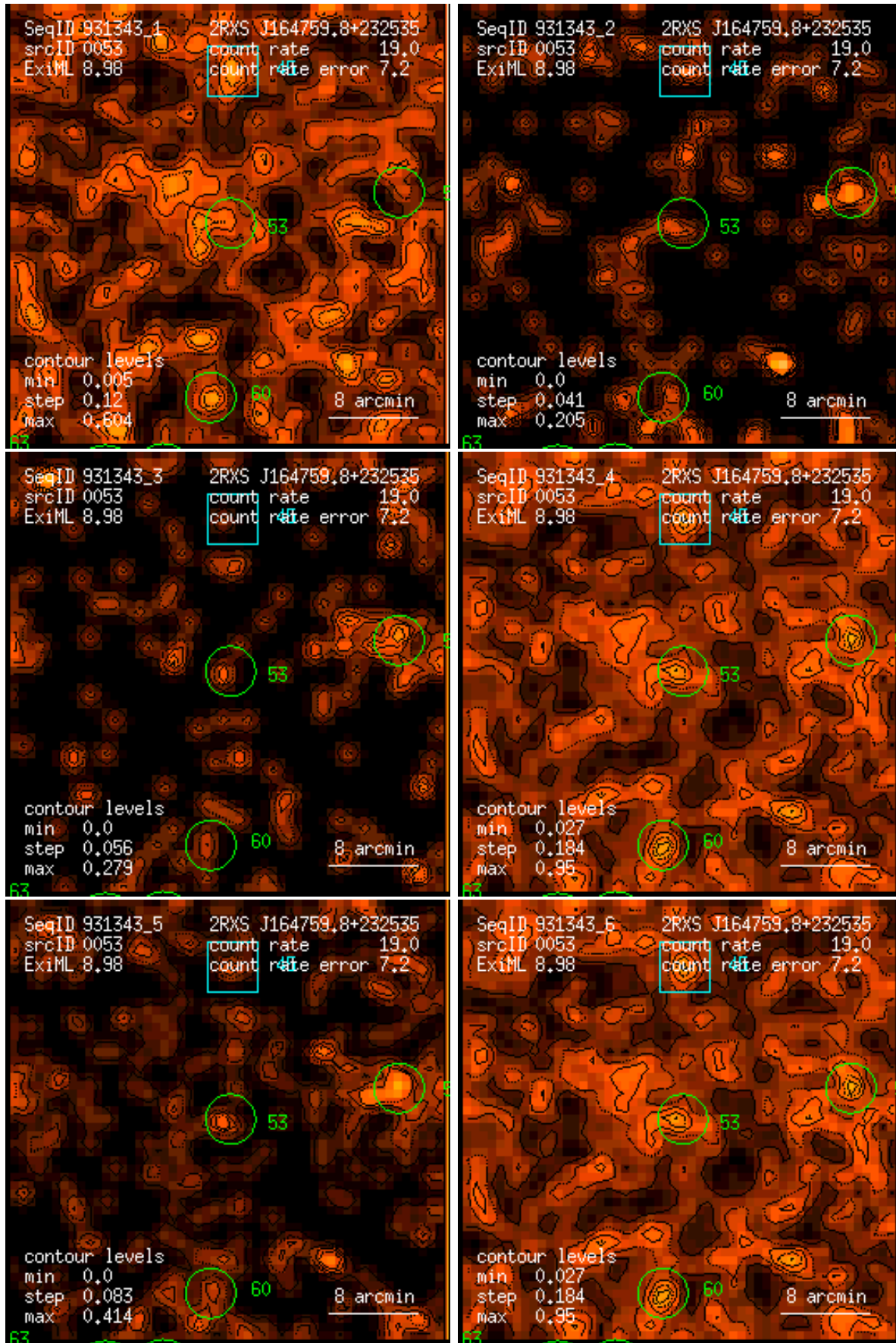
Figure 53: RASS 931343: detection 0053: band rate images, Gaussian filter: (1) PSPC channels 11 – 41, (2) 52 – 90, (3) 91 – 201, (4) 11 – 235, (5) 52 – 201, (6) 11 – 201. Broad band rates in counts/ks. Band rate contour levels in counts/ks/arcmin 2 .
