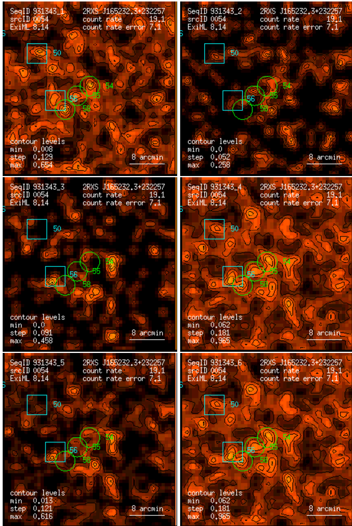
Figure 54: RASS 931343: detection 0054: band rate images, Gaussian filter: (1) PSPC channels 11 – 41, (2) 52 – 90, (3) 91 – 201, (4) 11 – 235, (5) 52 – 201, (6) 11 – 201. Broad band rates in counts/ks. Band rate contour levels in counts/ks/arcmin 2 .
