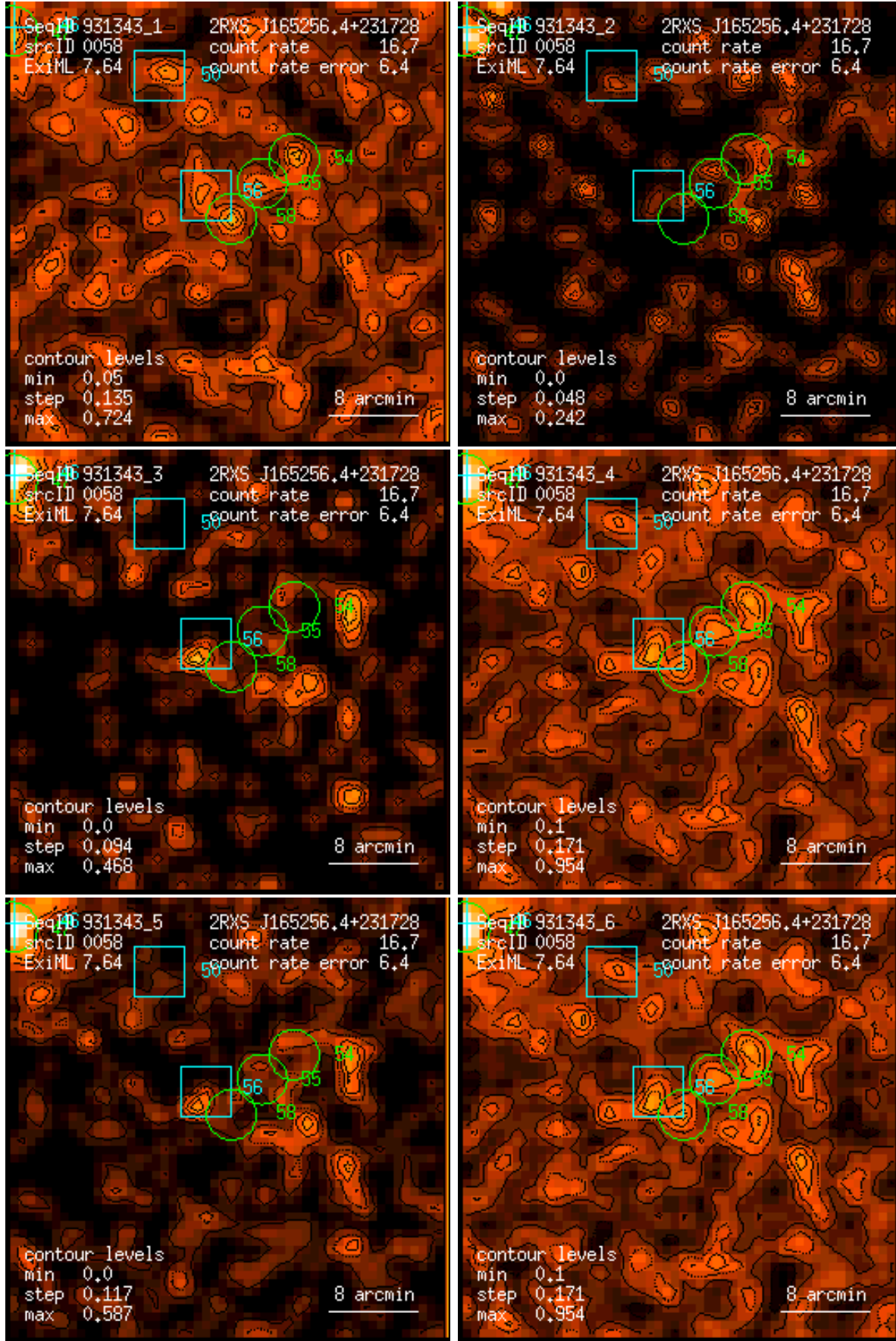
Figure 58: RASS 931343: detection 0058: band rate images, Gaussian filter: (1) PSPC channels 11 – 41, (2) 52 – 90, (3) 91 – 201, (4) 11 – 235, (5) 52 – 201, (6) 11 – 201. Broad band rates in counts/ks. Band rate contour levels in counts/ks/arcmin 2 .
