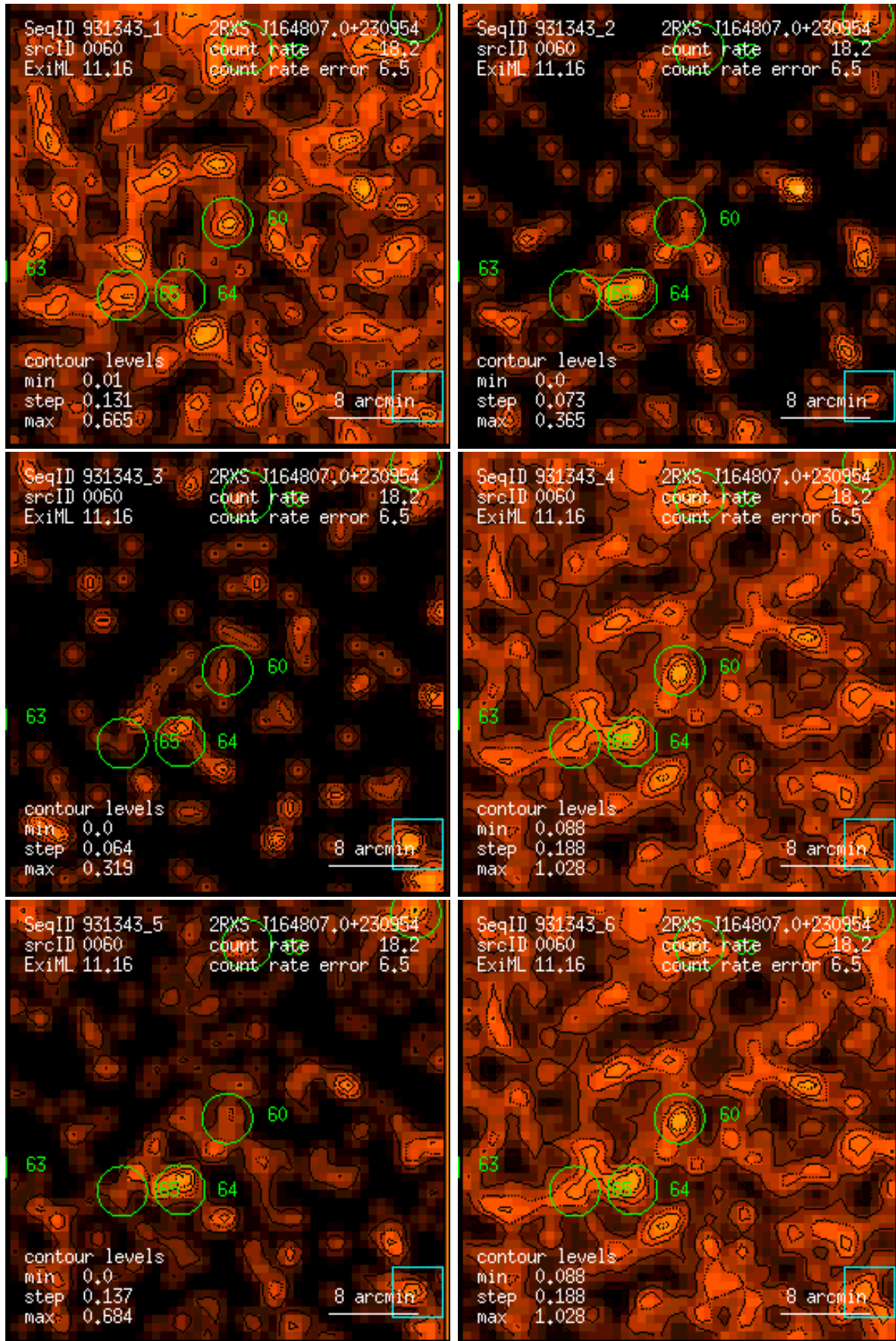
Figure 60: RASS 931343: detection 0060: band rate images, Gaussian filter: (1) PSPC channels 11 – 41, (2) 52 – 90, (3) 91 – 201, (4) 11 – 235, (5) 52 – 201, (6) 11 – 201. Broad band rates in counts/ks. Band rate contour levels in counts/ks/arcmin 2 .
