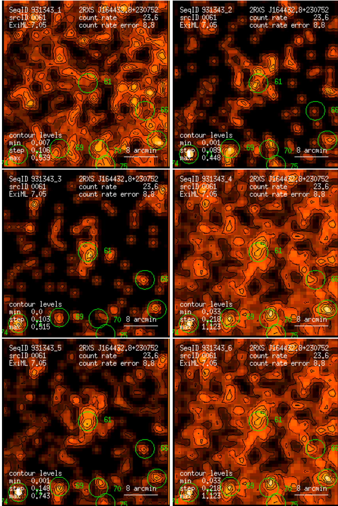
Figure 61: RASS 931343: detection 0061: band rate images, Gaussian filter: (1) PSPC channels 11 – 41, (2) 52 – 90, (3) 91 – 201, (4) 11 – 235, (5) 52 – 201, (6) 11 – 201. Broad band rates in counts/ks. Band rate contour levels in counts/ks/arcmin 2 .
