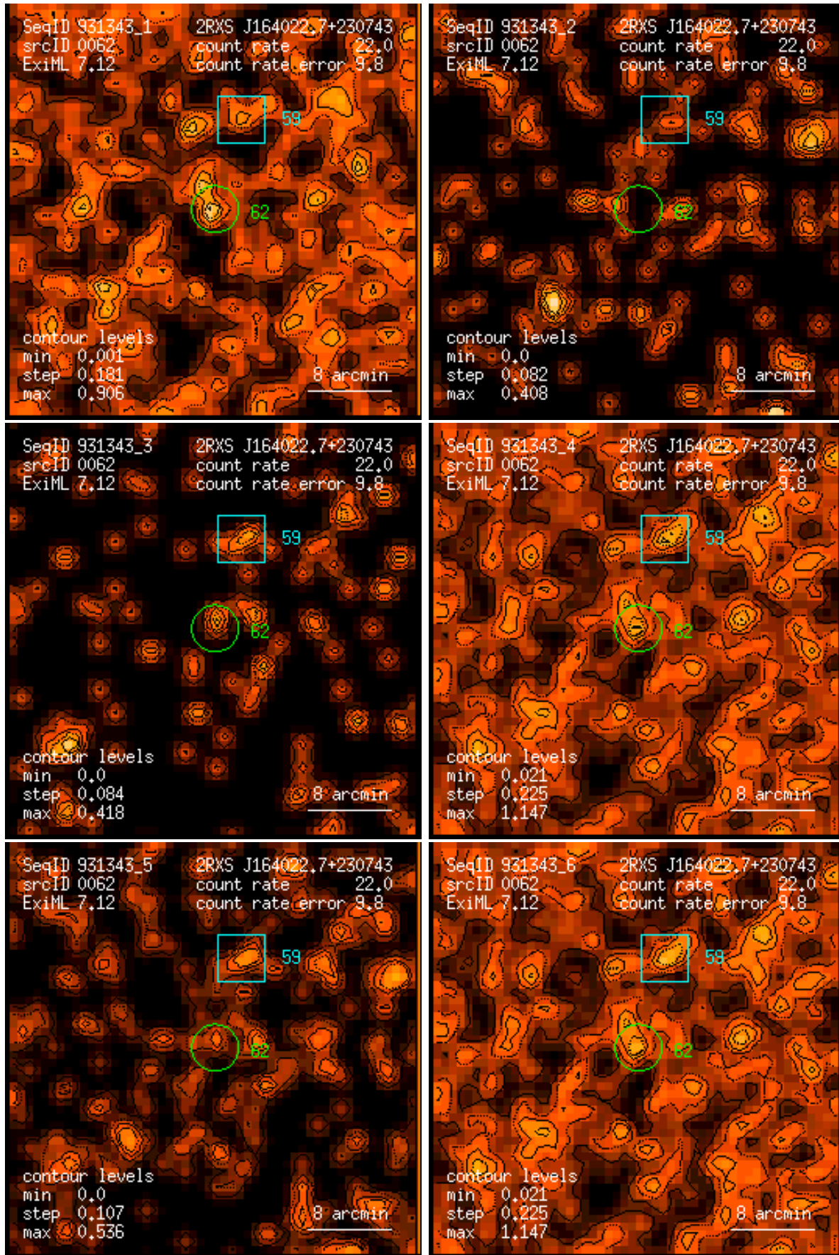
Figure 62: RASS 931343: detection 0062: band rate images, Gaussian filter: (1) PSPC channels 11 – 41, (2) 52 – 90, (3) 91 – 201, (4) 11 – 235, (5) 52 – 201, (6) 11 – 201. Broad band rates in counts/ks. Band rate contour levels in counts/ks/arcmin 2 .
