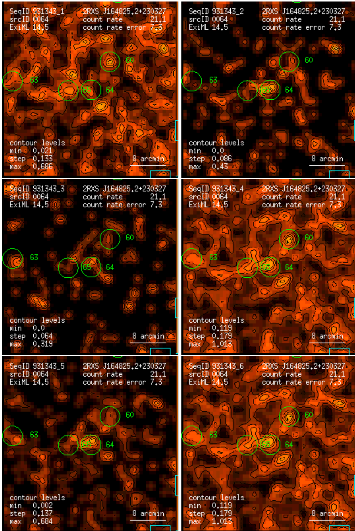
Figure 64: RASS 931343: detection 0064: band rate images, Gaussian filter: (1) PSPC channels 11 – 41, (2) 52 – 90, (3) 91 – 201, (4) 11 – 235, (5) 52 – 201, (6) 11 – 201. Broad band rates in counts/ks. Band rate contour levels in counts/ks/arcmin 2 .
