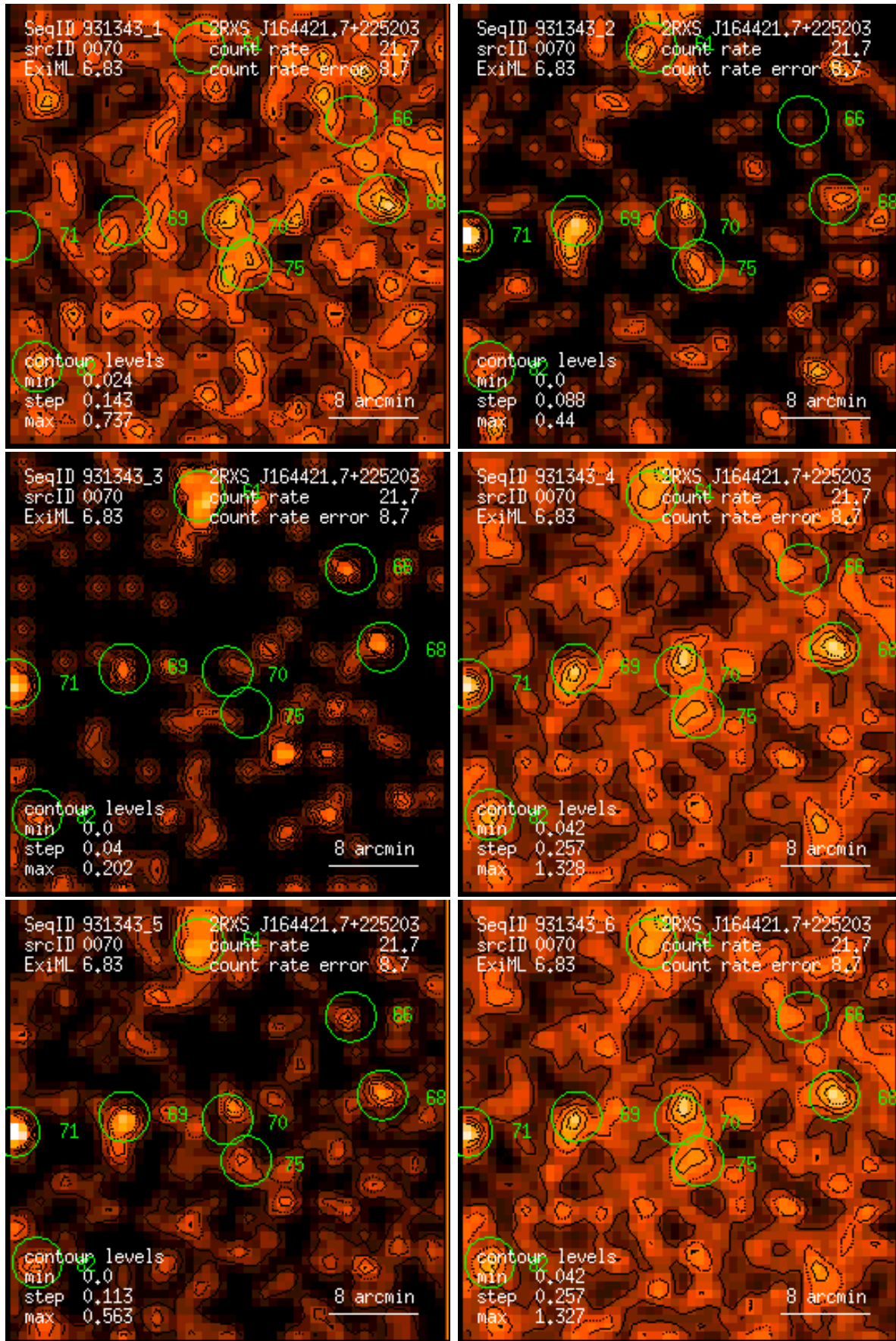
Figure 70: RASS 931343: detection 0070: band rate images, Gaussian filter: (1) PSPC channels 11 – 41, (2) 52 – 90, (3) 91 – 201, (4) 11 – 235, (5) 52 – 201, (6) 11 – 201. Broad band rates in counts/ks. Band rate contour levels in counts/ks/arcmin 2 .
