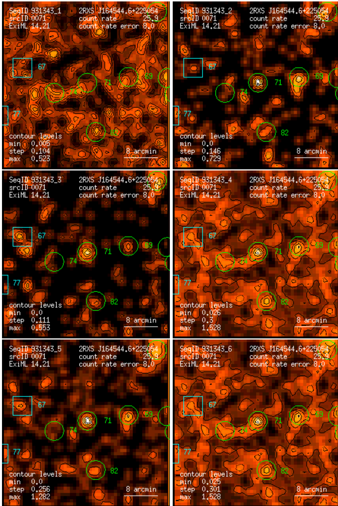
Figure 71: RASS 931343: detection 0071: band rate images, Gaussian filter: (1) PSPC channels 11 – 41, (2) 52 – 90, (3) 91 – 201, (4) 11 – 235, (5) 52 – 201, (6) 11 – 201. Broad band rates in counts/ks. Band rate contour levels in counts/ks/arcmin 2 .
