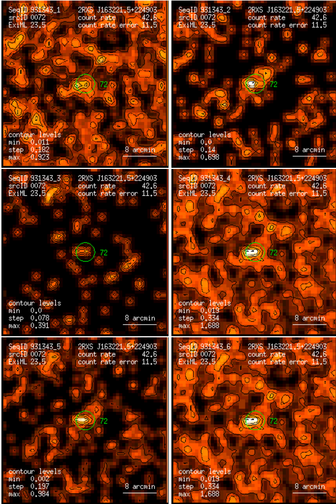
Figure 72: RASS 931343: detection 0072: band rate images, Gaussian filter: (1) PSPC channels 11 – 41, (2) 52 – 90, (3) 91 – 201, (4) 11 – 235, (5) 52 – 201, (6) 11 – 201. Broad band rates in counts/ks. Band rate contour levels in counts/ks/arcmin 2 .
