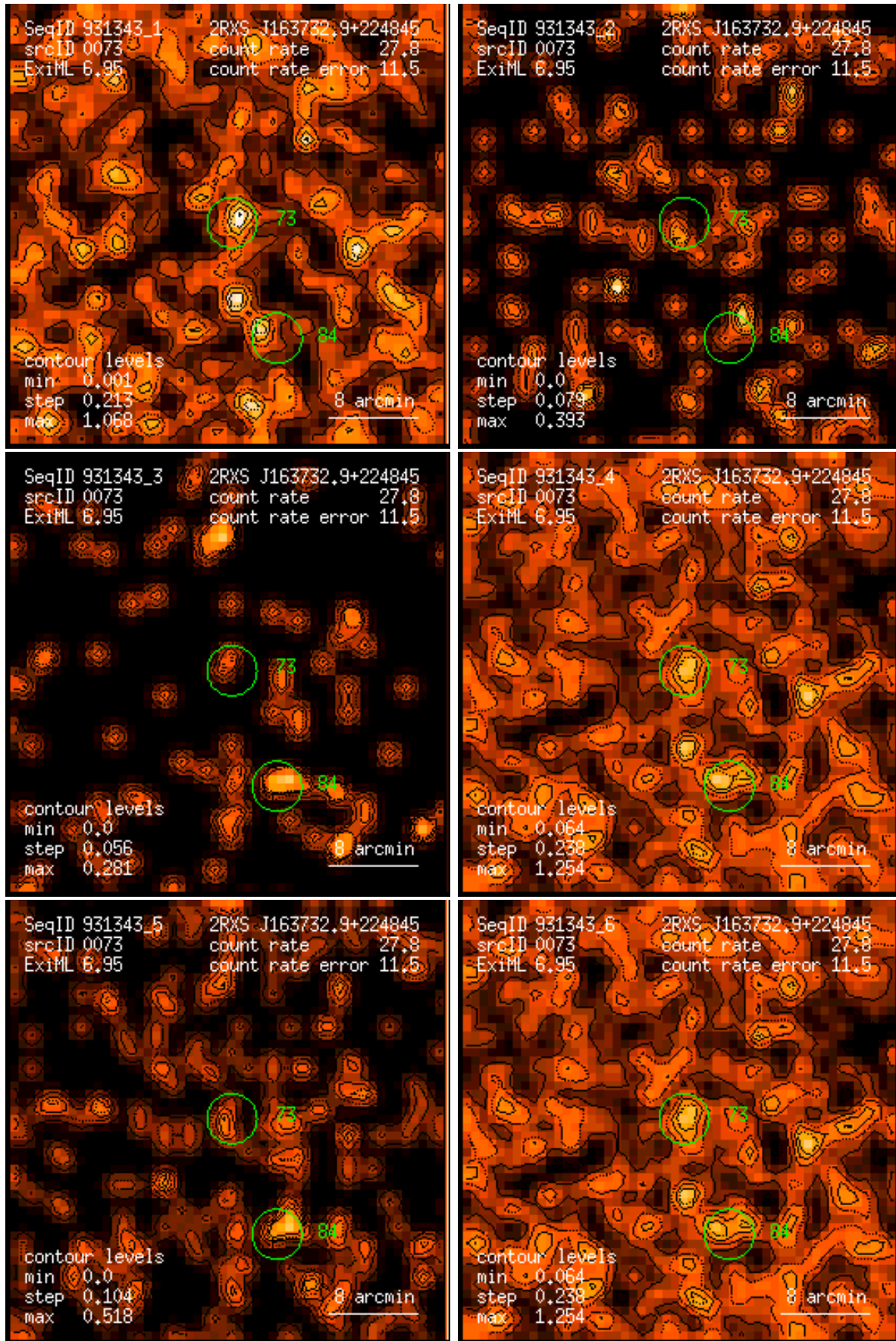
Figure 73: RASS 931343: detection 0073: band rate images, Gaussian filter: (1) PSPC channels 11 – 41, (2) 52 – 90, (3) 91 – 201, (4) 11 – 235, (5) 52 – 201, (6) 11 – 201. Broad band rates in counts/ks. Band rate contour levels in counts/ks/arcmin 2 .
