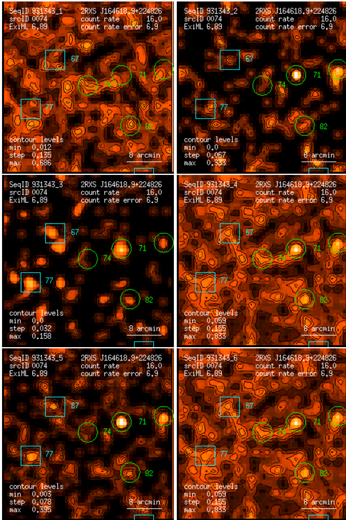
Figure 74: RASS 931343: detection 0074: band rate images, Gaussian filter: (1) PSPC channels 11 – 41, (2) 52 – 90, (3) 91 – 201, (4) 11 – 235, (5) 52 – 201, (6) 11 – 201. Broad band rates in counts/ks. Band rate contour levels in counts/ks/arcmin 2 .
