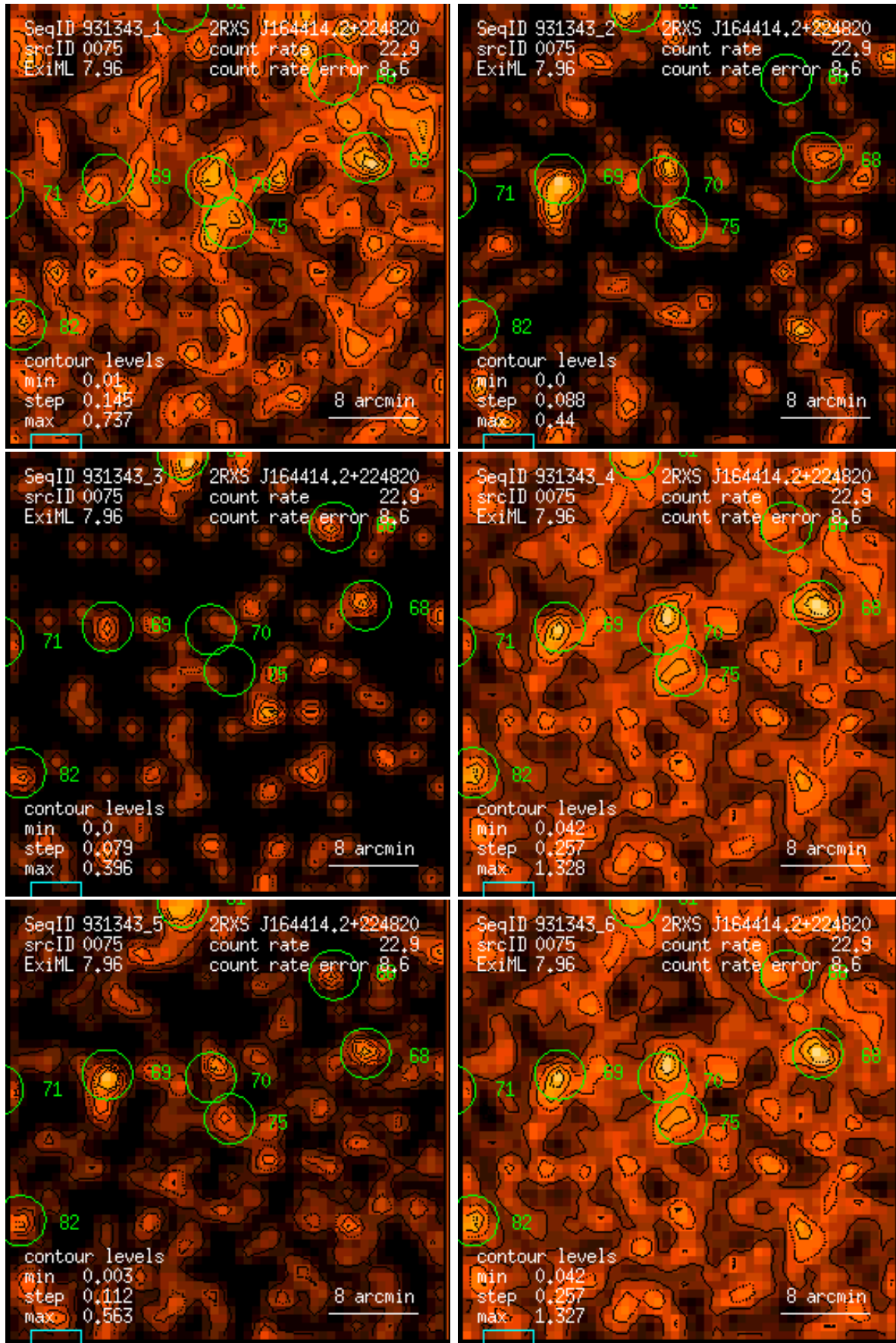
Figure 75: RASS 931343: detection 0075: band rate images, Gaussian filter: (1) PSPC channels 11 – 41, (2) 52 – 90, (3) 91 – 201, (4) 11 – 235, (5) 52 – 201, (6) 11 – 201. Broad band rates in counts/ks. Band rate contour levels in counts/ks/arcmin 2 .
