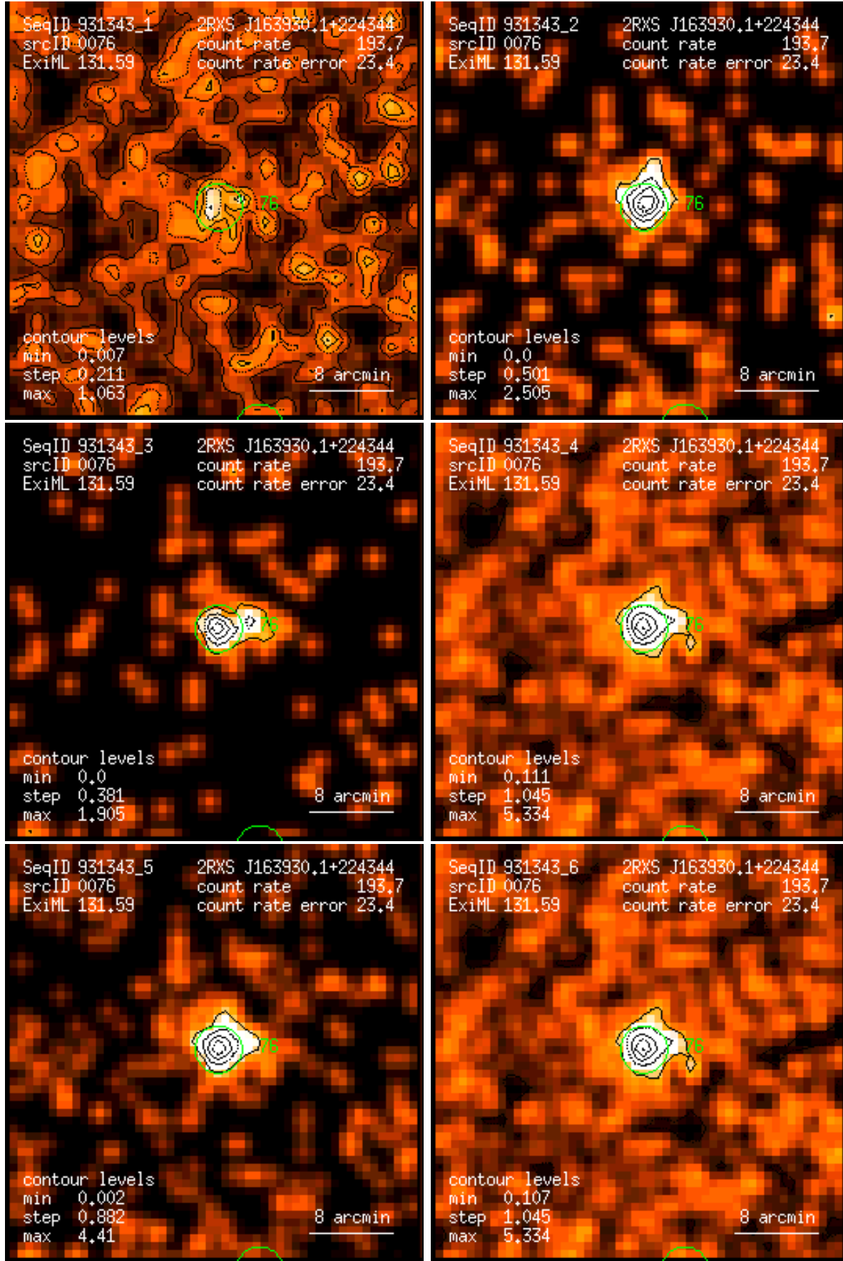
Figure 76: RASS 931343: detection 0076: band rate images, Gaussian filter: (1) PSPC channels 11 – 41, (2) 52 – 90, (3) 91 – 201, (4) 11 – 235, (5) 52 – 201, (6) 11 – 201. Broad band rates in counts/ks. Band rate contour levels in counts/ks/arcmin 2 .
