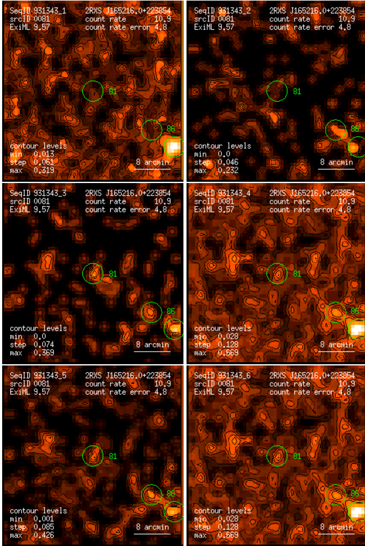
Figure 81: RASS 931343: detection 0081: band rate images, Gaussian filter: (1) PSPC channels 11 – 41, (2) 52 – 90, (3) 91 – 201, (4) 11 – 235, (5) 52 – 201, (6) 11 – 201. Broad band rates in counts/ks. Band rate contour levels in counts/ks/arcmin 2 .
