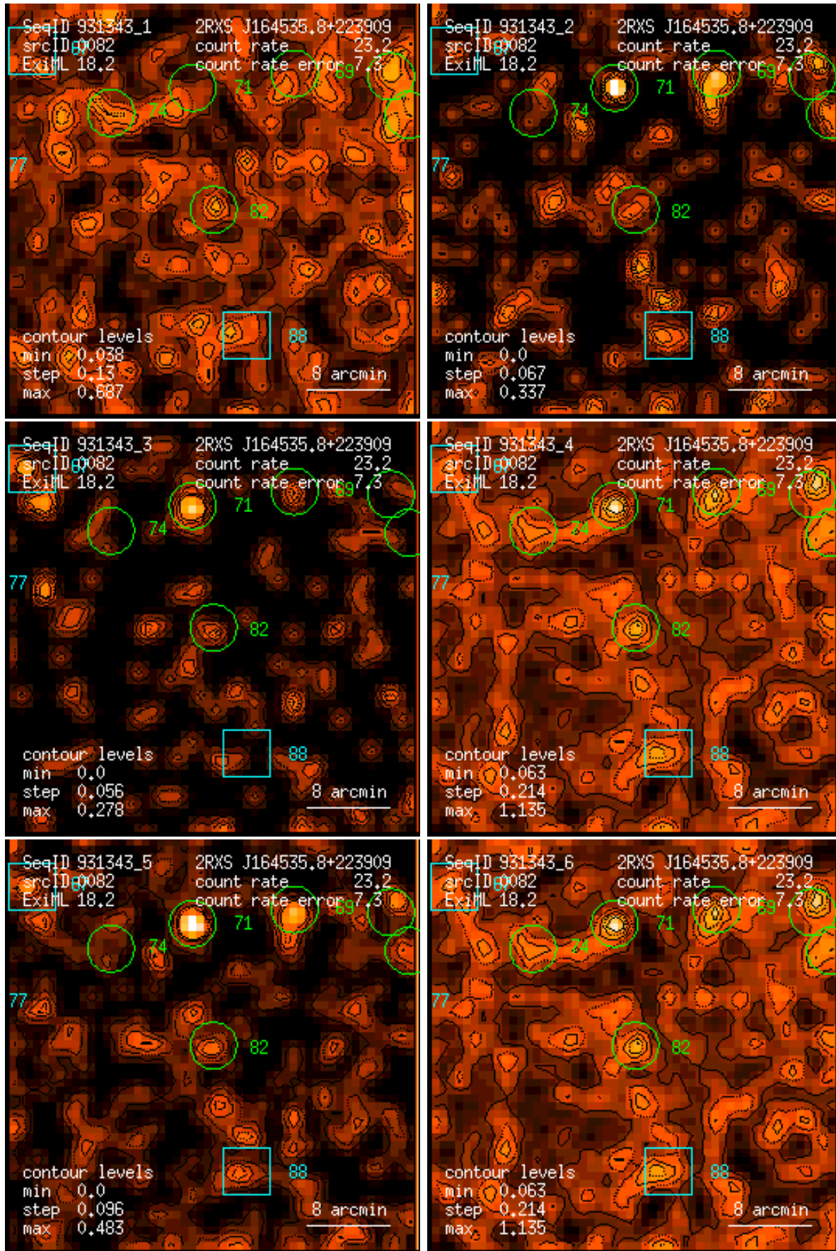
Figure 82: RASS 931343: detection 0082: band rate images, Gaussian filter: (1) PSPC channels 11 – 41, (2) 52 – 90, (3) 91 – 201, (4) 11 – 235, (5) 52 – 201, (6) 11 – 201. Broad band rates in counts/ks. Band rate contour levels in counts/ks/arcmin 2 .
