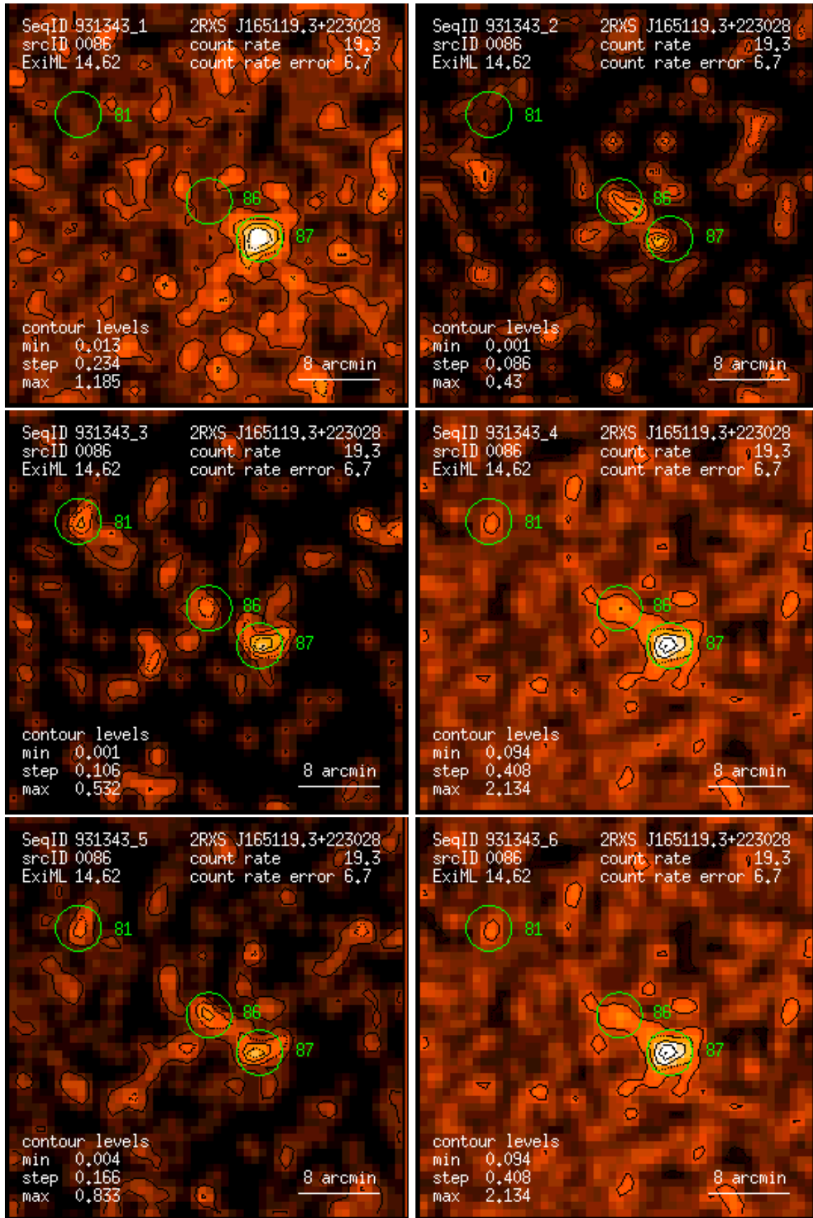
Figure 86: RASS 931343: detection 0086: band rate images, Gaussian filter: (1) PSPC channels 11 – 41, (2) 52 – 90, (3) 91 – 201, (4) 11 – 235, (5) 52 – 201, (6) 11 – 201. Broad band rates in counts/ks. Band rate contour levels in counts/ks/arcmin 2 .
