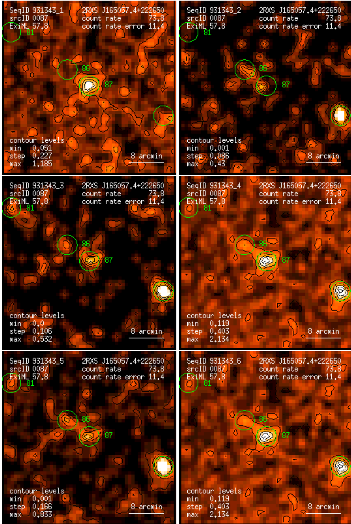
Figure 87: RASS 931343: detection 0087: band rate images, Gaussian filter: (1) PSPC channels 11 – 41, (2) 52 – 90, (3) 91 – 201, (4) 11 – 235, (5) 52 – 201, (6) 11 – 201. Broad band rates in counts/ks. Band rate contour levels in counts/ks/arcmin 2 .
