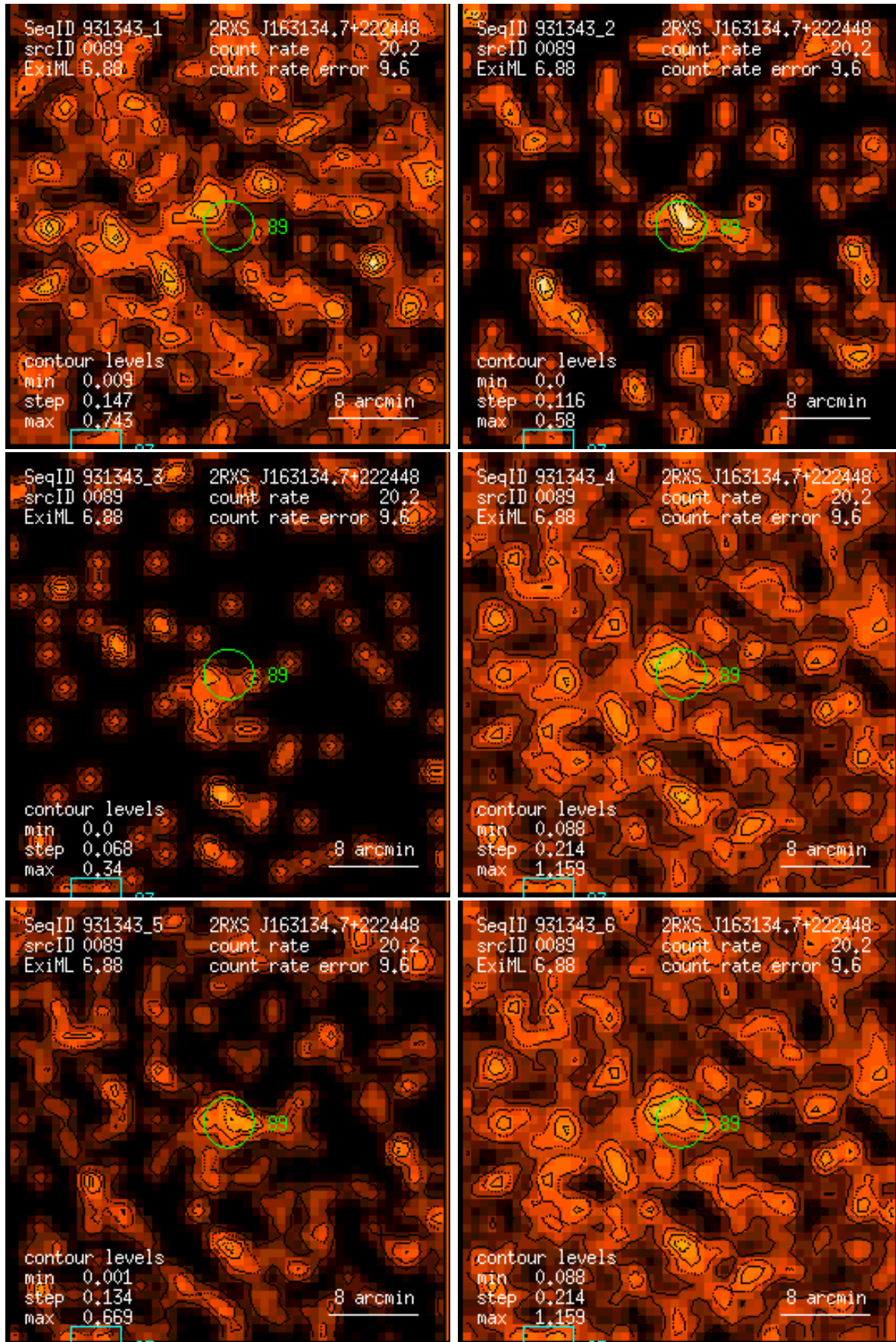
Figure 89: RASS 931343: detection 0089: band rate images, Gaussian filter: (1) PSPC channels 11 – 41, (2) 52 – 90, (3) 91 – 201, (4) 11 – 235, (5) 52 – 201, (6) 11 – 201. Broad band rates in counts/ks. Band rate contour levels in counts/ks/arcmin 2 .
