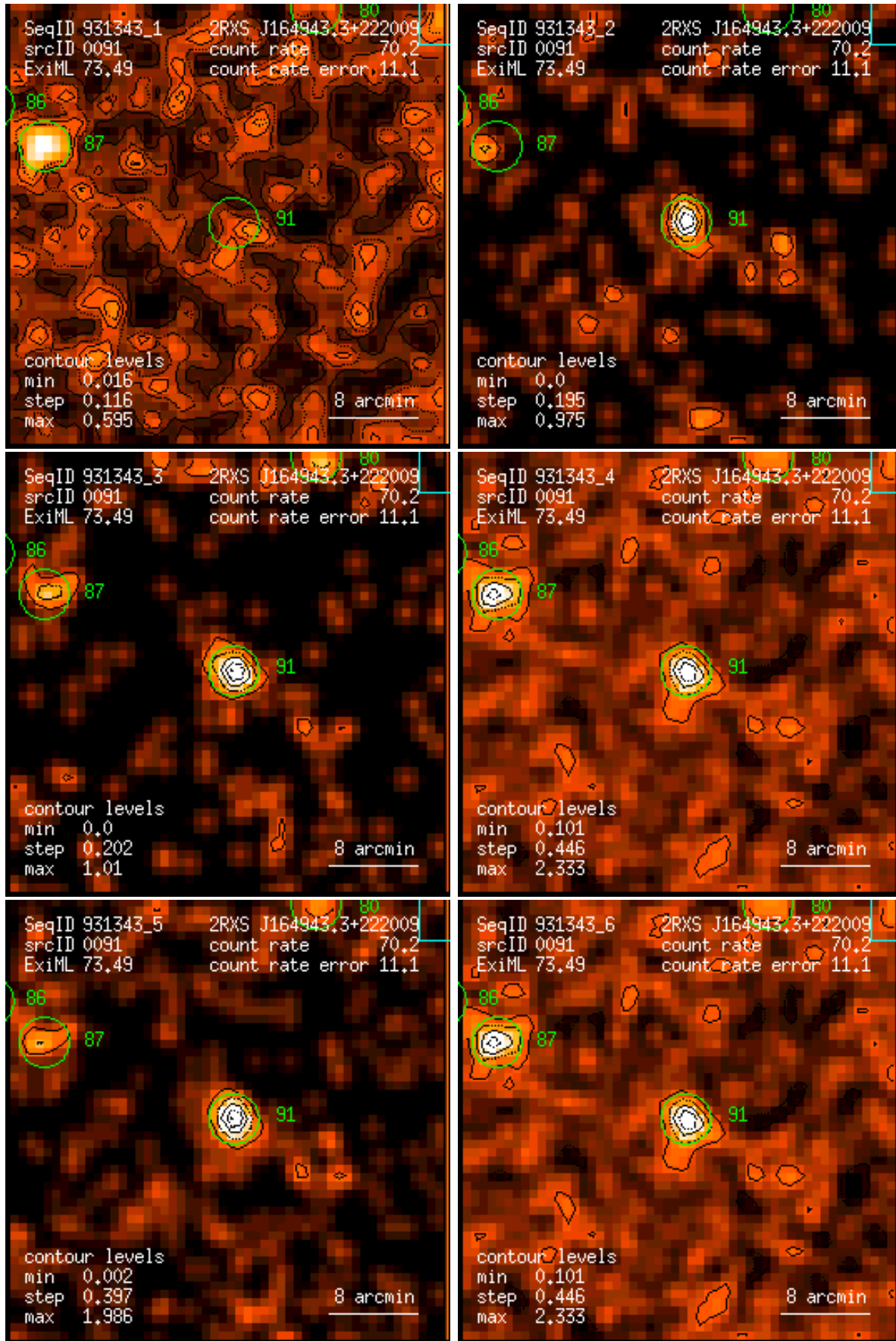
Figure 91: RASS 931343: detection 0091: band rate images, Gaussian filter: (1) PSPC channels 11 – 41, (2) 52 – 90, (3) 91 – 201, (4) 11 – 235, (5) 52 – 201, (6) 11 – 201. Broad band rates in counts/ks. Band rate contour levels in counts/ks/arcmin 2 .
