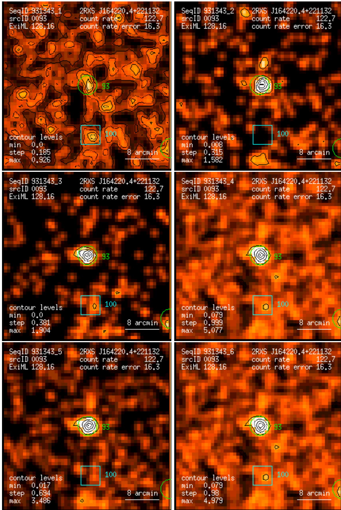
Figure 93: RASS 931343: detection 0093: band rate images, Gaussian filter: (1) PSPC channels 11 – 41, (2) 52 – 90, (3) 91 – 201, (4) 11 – 235, (5) 52 – 201, (6) 11 – 201. Broad band rates in counts/ks. Band rate contour levels in counts/ks/arcmin 2 .
