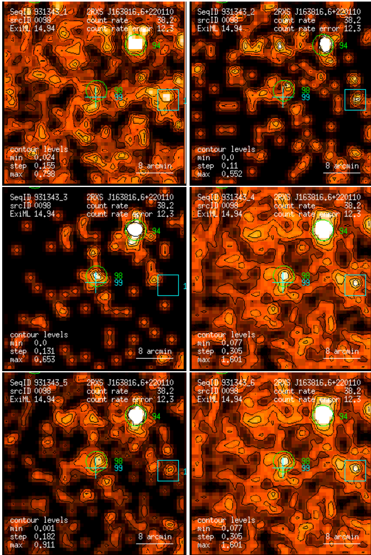
Figure 98: RASS 931343: detection 0098: band rate images, Gaussian filter: (1) PSPC channels 11 – 41, (2) 52 – 90, (3) 91 – 201, (4) 11 – 235, (5) 52 – 201, (6) 11 – 201. Broad band rates in counts/ks. Band rate contour levels in counts/ks/arcmin 2 .
