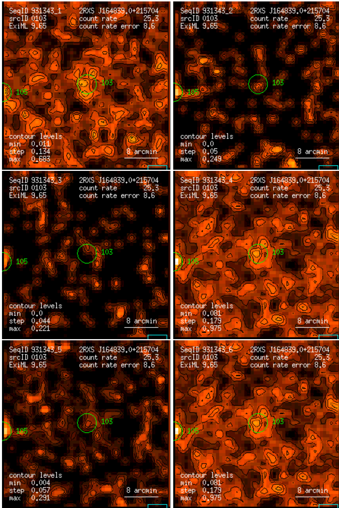
Figure 103: RASS 931343: detection 0103: band rate images, Gaussian filter: (1) PSPC channels 11 – 41, (2) 52 – 90, (3) 91 – 201, (4) 11 – 235, (5) 52 – 201, (6) 11 – 201. Broad band rates in counts/ks. Band rate contour levels in counts/ks/arcmin 2 .
