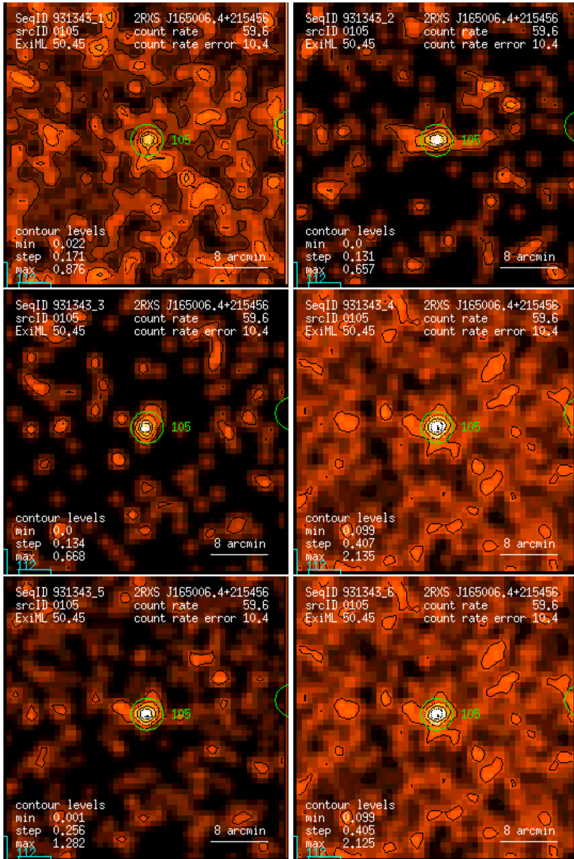
Figure 105: RASS 931343: detection 0105: band rate images, Gaussian filter: (1) PSPC channels 11 – 41, (2) 52 – 90, (3) 91 – 201, (4) 11 – 235, (5) 52 – 201, (6) 11 – 201. Broad band rates in counts/ks. Band rate contour levels in counts/ks/arcmin 2 .
