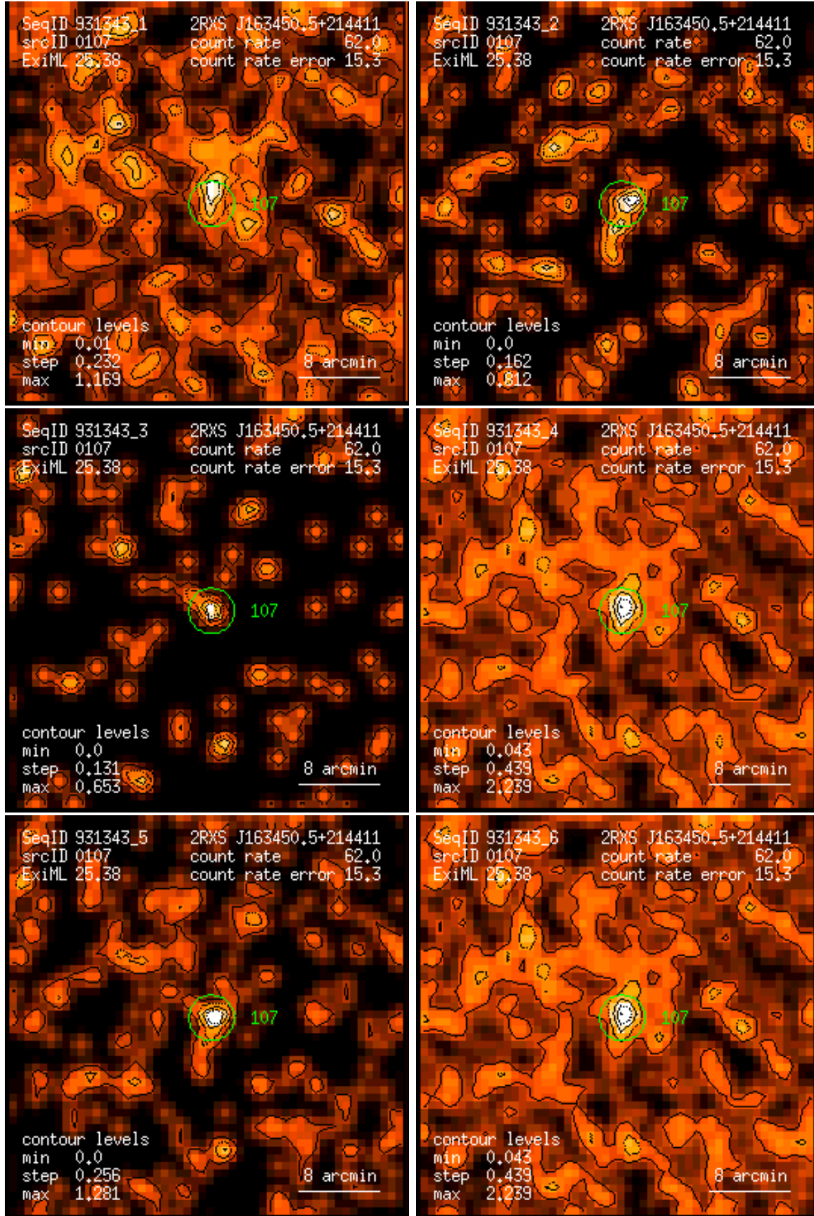
Figure 107: RASS 931343: detection 0107: band rate images, Gaussian filter: (1) PSPC channels 11 – 41, (2) 52 – 90, (3) 91 – 201, (4) 11 – 235, (5) 52 – 201, (6) 11 – 201. Broad band rates in counts/ks. Band rate contour levels in counts/ks/arcmin 2 .
