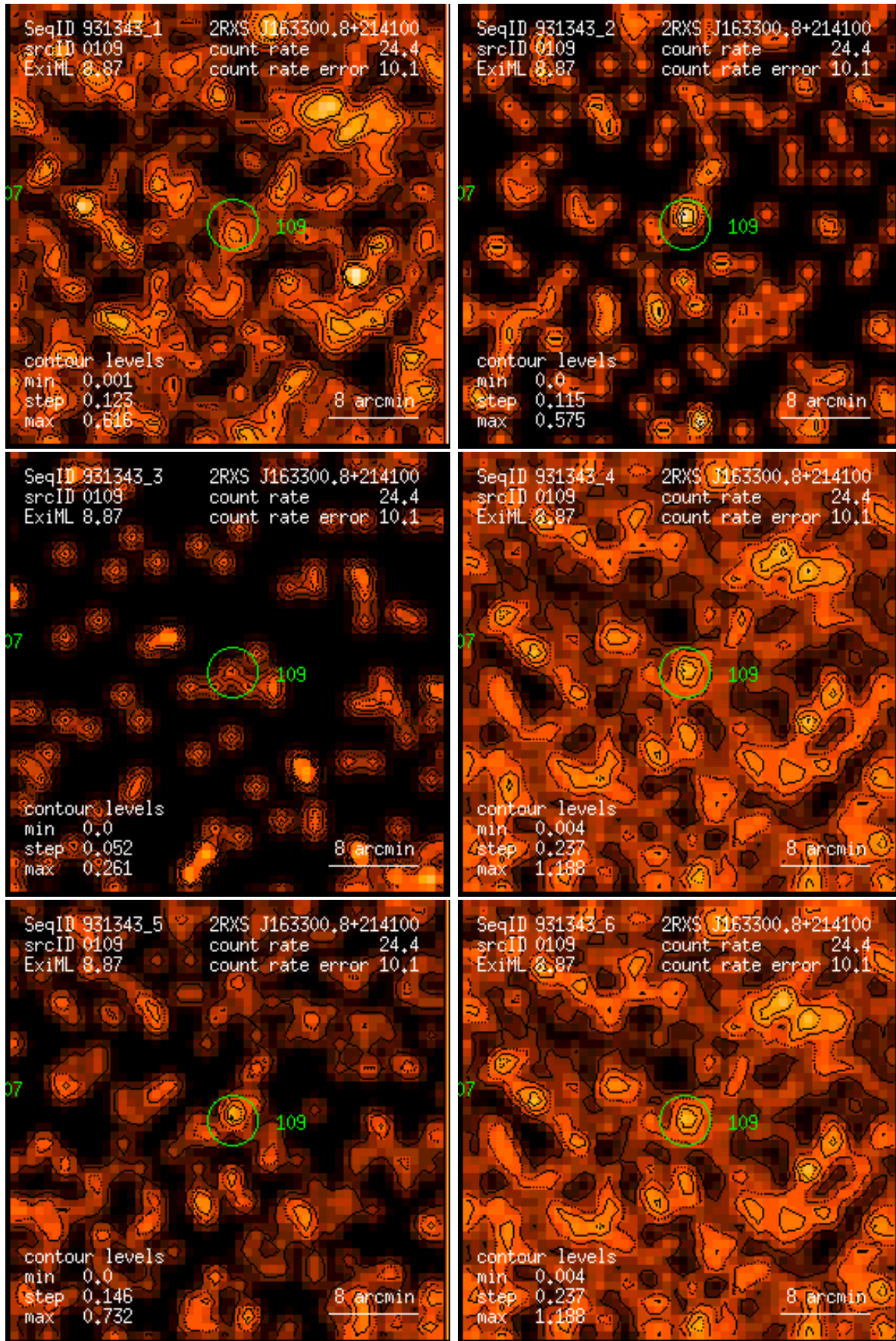
Figure 109: RASS 931343: detection 0109: band rate images, Gaussian filter: (1) PSPC channels 11 – 41, (2) 52 – 90, (3) 91 – 201, (4) 11 – 235, (5) 52 – 201, (6) 11 – 201. Broad band rates in counts/ks. Band rate contour levels in counts/ks/arcmin 2 .
