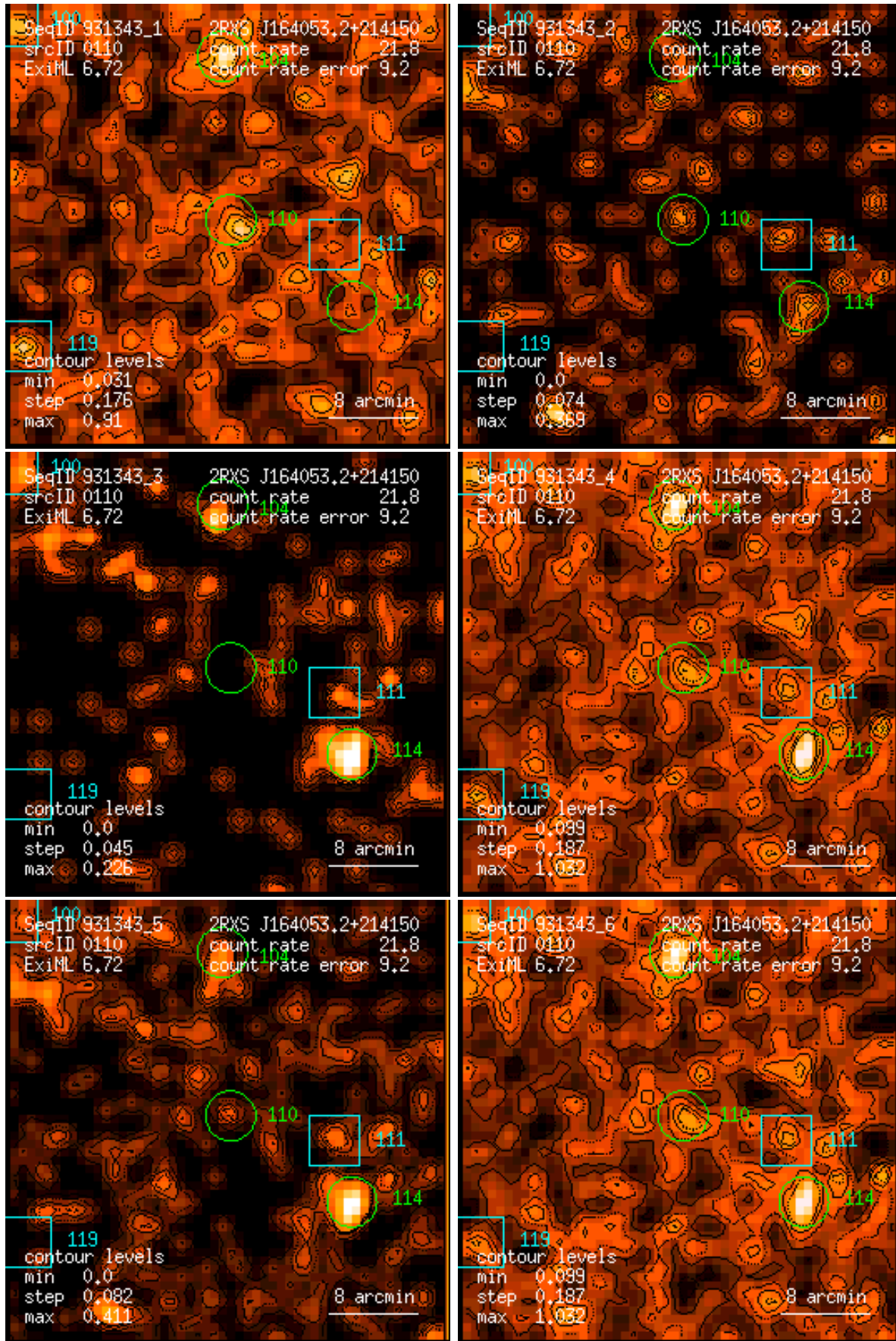
Figure 110: RASS 931343: detection 0110: band rate images, Gaussian filter: (1) PSPC channels 11 – 41, (2) 52 – 90, (3) 91 – 201, (4) 11 – 235, (5) 52 – 201, (6) 11 – 201. Broad band rates in counts/ks. Band rate contour levels in counts/ks/arcmin 2 .
