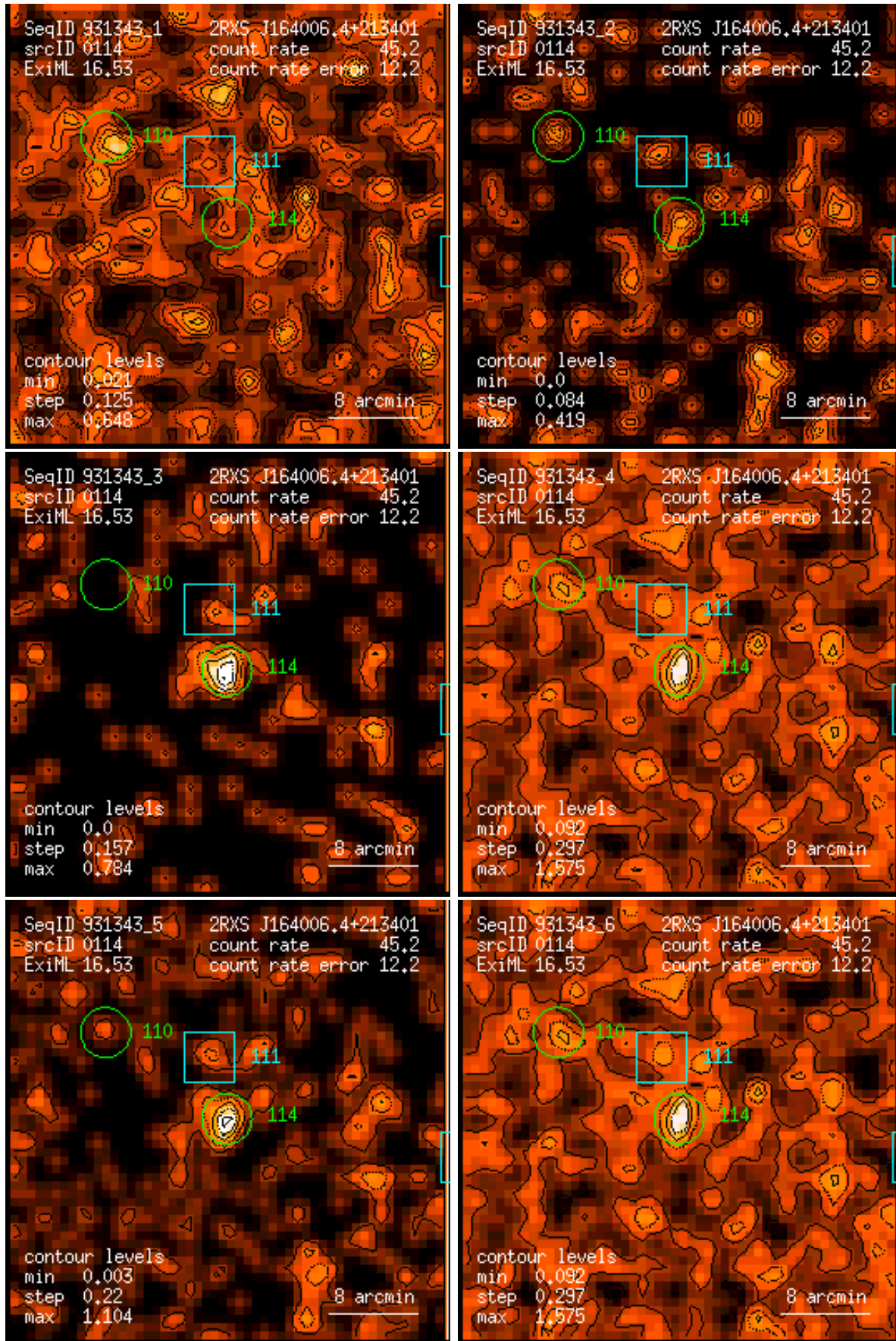
Figure 114: RASS 931343: detection 0114: band rate images, Gaussian filter: (1) PSPC channels 11 – 41, (2) 52 – 90, (3) 91 – 201, (4) 11 – 235, (5) 52 – 201, (6) 11 – 201. Broad band rates in counts/ks. Band rate contour levels in counts/ks/arcmin 2 .
