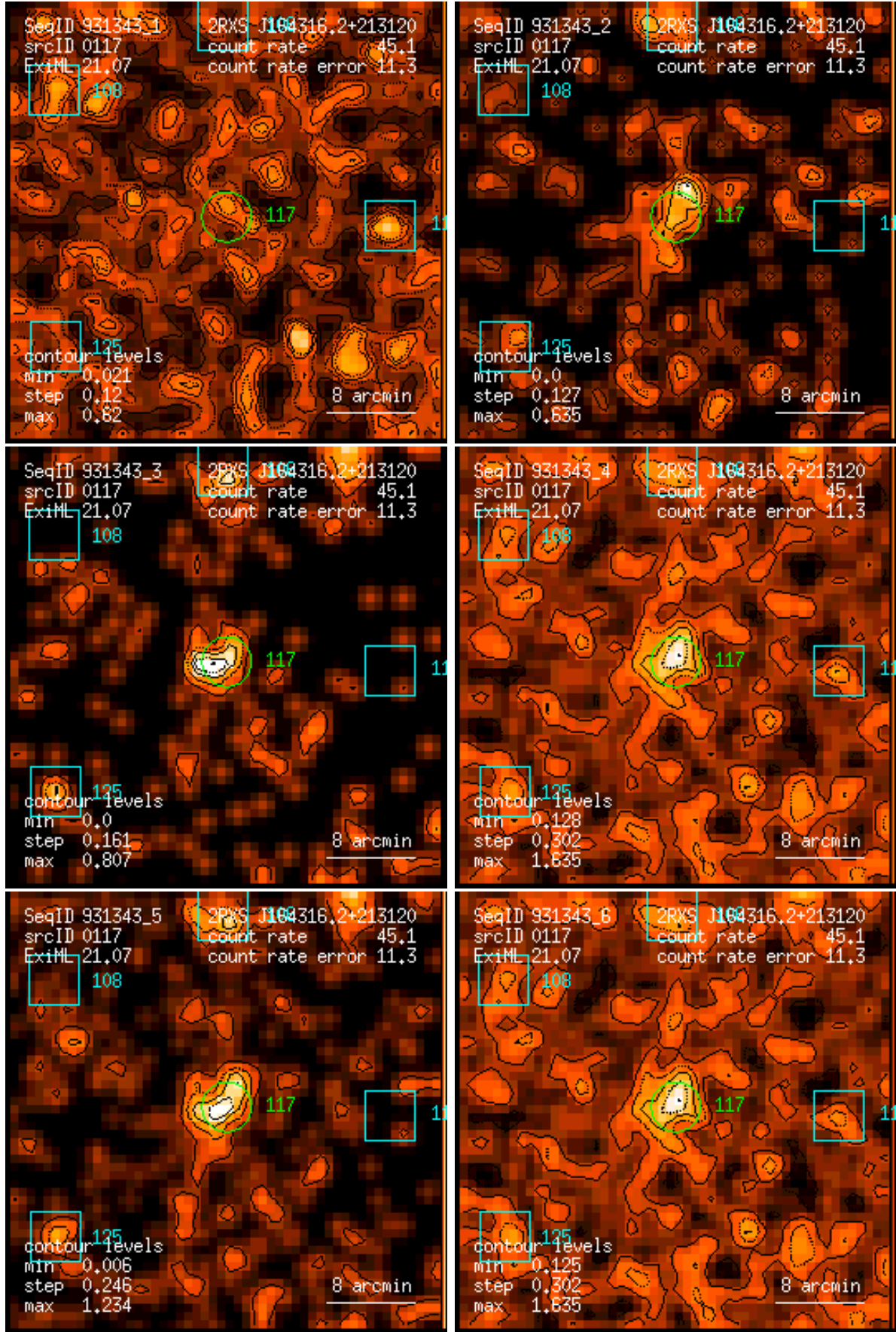
Figure 117: RASS 931343: detection 0117: band rate images, Gaussian filter: (1) PSPC channels 11 – 41, (2) 52 – 90, (3) 91 – 201, (4) 11 – 235, (5) 52 – 201, (6) 11 – 201. Broad band rates in counts/ks. Band rate contour levels in counts/ks/arcmin 2 .
