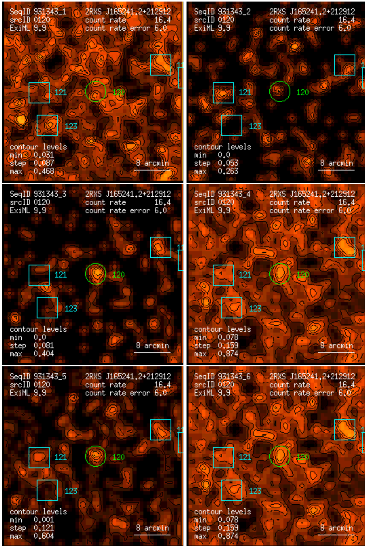
Figure 120: RASS 931343: detection 0120: band rate images, Gaussian filter: (1) PSPC channels 11 – 41, (2) 52 – 90, (3) 91 – 201, (4) 11 – 235, (5) 52 – 201, (6) 11 – 201. Broad band rates in counts/ks. Band rate contour levels in counts/ks/arcmin 2 .
