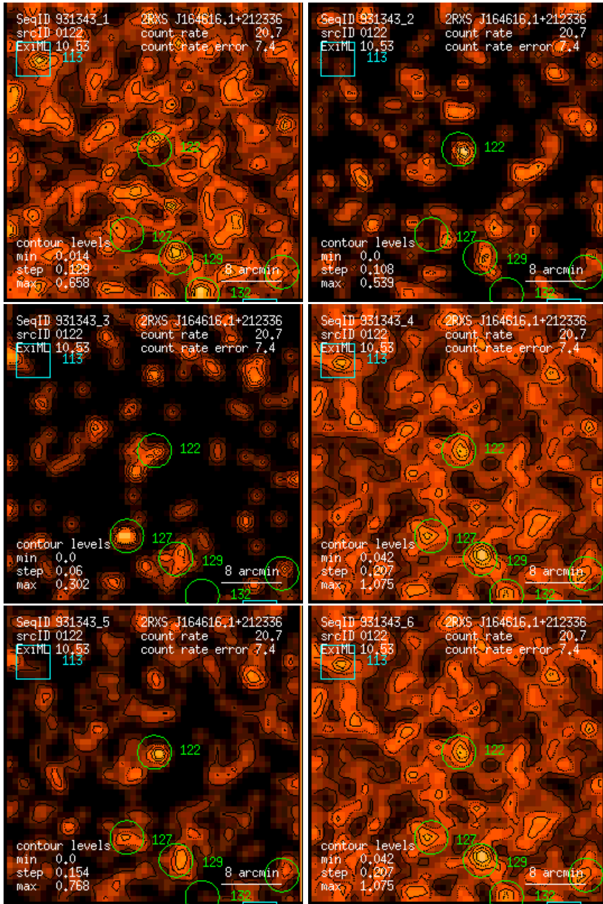
Figure 122: RASS 931343: detection 0122: band rate images, Gaussian filter: (1) PSPC channels 11 – 41, (2) 52 – 90, (3) 91 – 201, (4) 11 – 235, (5) 52 – 201, (6) 11 – 201. Broad band rates in counts/ks. Band rate contour levels in counts/ks/arcmin 2 .
