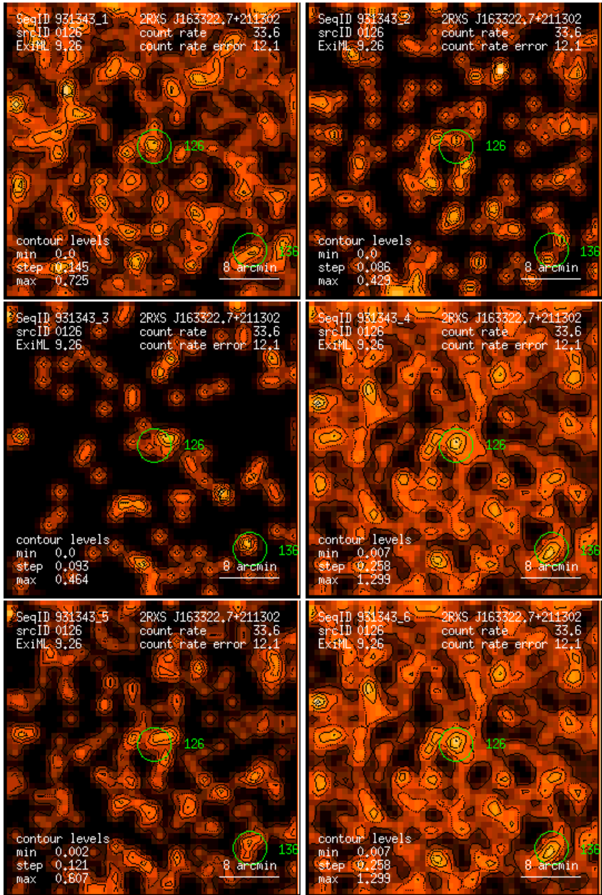
Figure 126: RASS 931343: detection 0126: band rate images, Gaussian filter: (1) PSPC channels 11 – 41, (2) 52 – 90, (3) 91 – 201, (4) 11 – 235, (5) 52 – 201, (6) 11 – 201. Broad band rates in counts/ks. Band rate contour levels in counts/ks/arcmin 2 .
