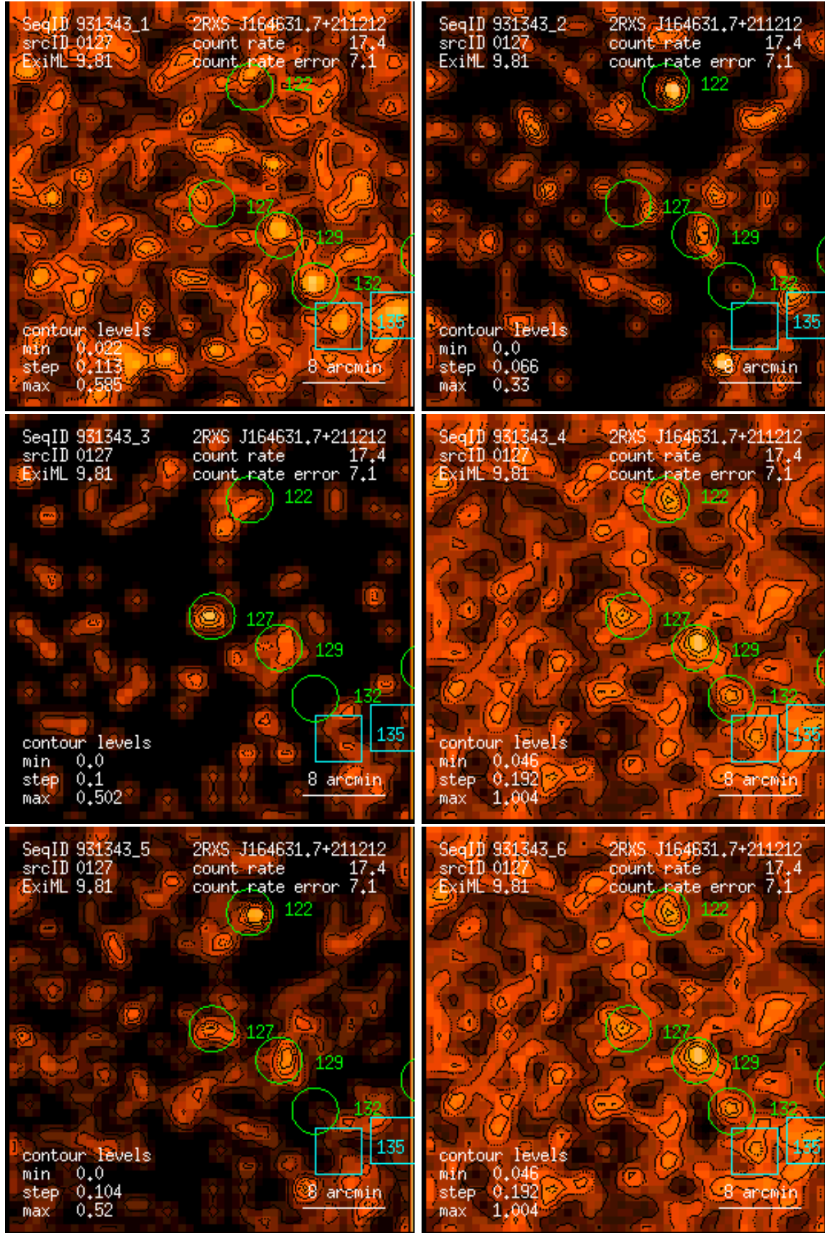
Figure 127: RASS 931343: detection 0127: band rate images, Gaussian filter: (1) PSPC channels 11 – 41, (2) 52 – 90, (3) 91 – 201, (4) 11 – 235, (5) 52 – 201, (6) 11 – 201. Broad band rates in counts/ks. Band rate contour levels in counts/ks/arcmin 2 .
