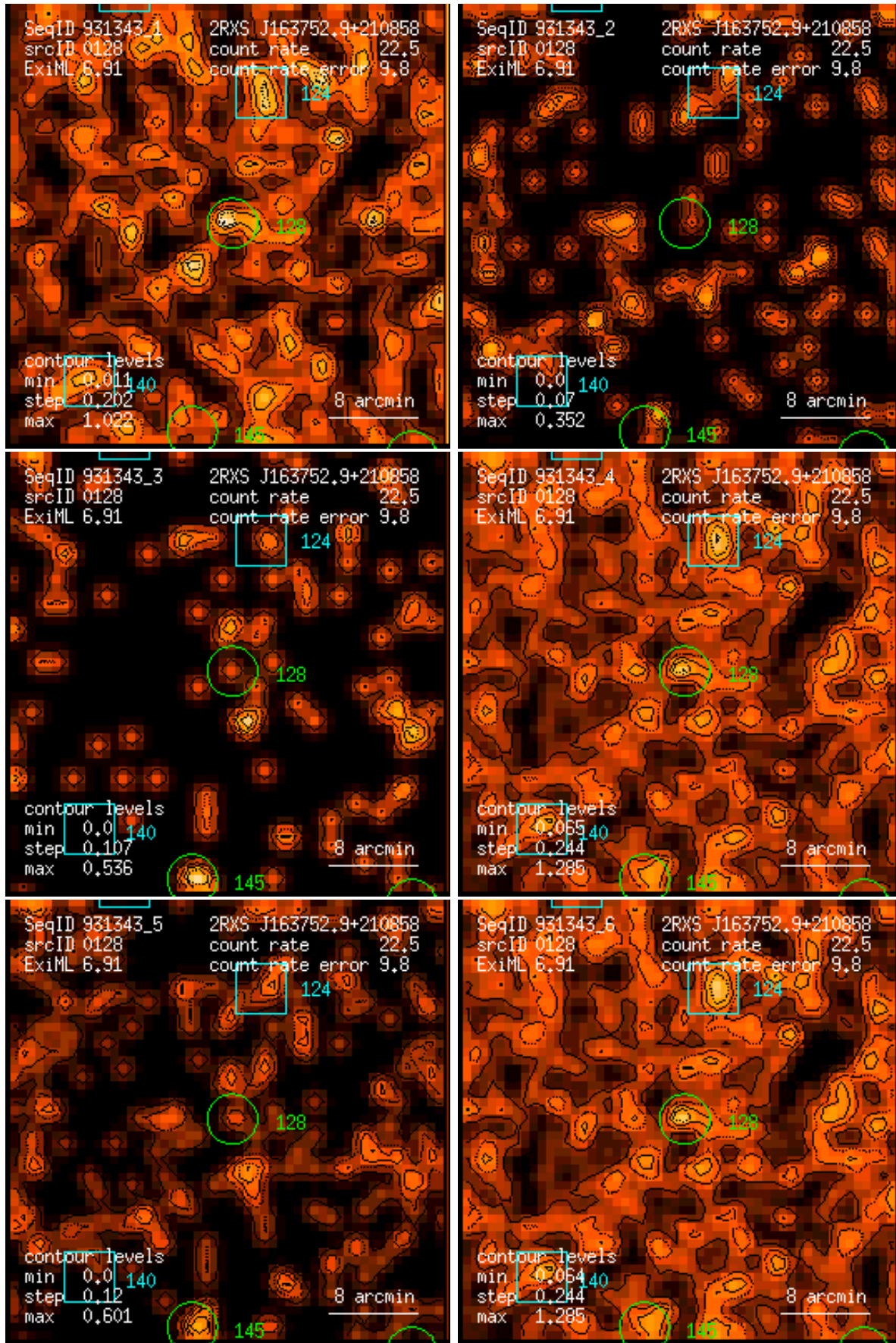
Figure 128: RASS 931343: detection 0128: band rate images, Gaussian filter: (1) PSPC channels 11 – 41, (2) 52 – 90, (3) 91 – 201, (4) 11 – 235, (5) 52 – 201, (6) 11 – 201. Broad band rates in counts/ks. Band rate contour levels in counts/ks/arcmin 2 .
