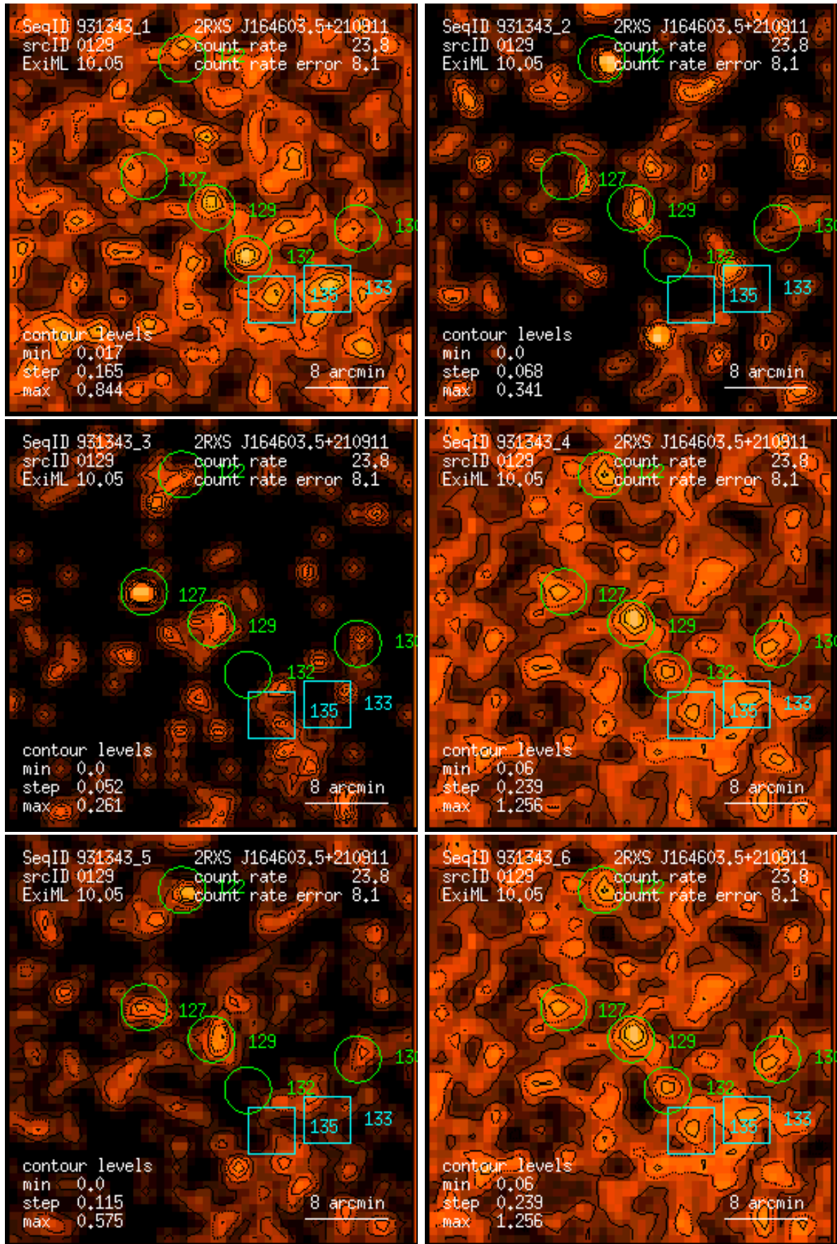
Figure 129: RASS 931343: detection 0129: band rate images, Gaussian filter: (1) PSPC channels 11 – 41, (2) 52 – 90, (3) 91 – 201, (4) 11 – 235, (5) 52 – 201, (6) 11 – 201. Broad band rates in counts/ks. Band rate contour levels in counts/ks/arcmin 2 .
