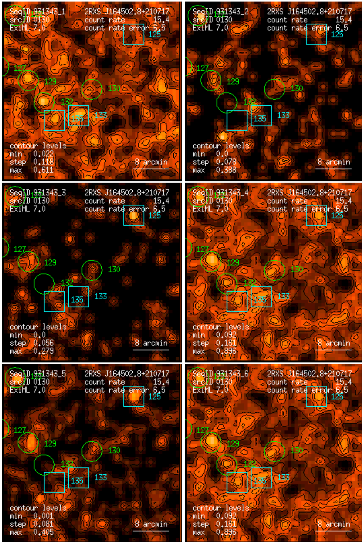
Figure 130: RASS 931343: detection 0130: band rate images, Gaussian filter: (1) PSPC channels 11 – 41, (2) 52 – 90, (3) 91 – 201, (4) 11 – 235, (5) 52 – 201, (6) 11 – 201. Broad band rates in counts/ks. Band rate contour levels in counts/ks/arcmin 2 .
