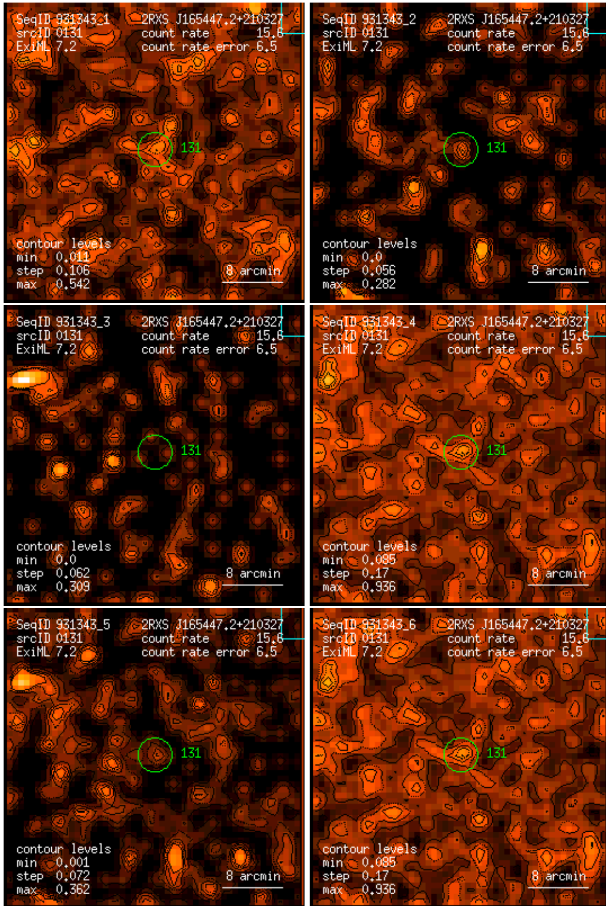
Figure 131: RASS 931343: detection 0131: band rate images, Gaussian filter: (1) PSPC channels 11 – 41, (2) 52 – 90, (3) 91 – 201, (4) 11 – 235, (5) 52 – 201, (6) 11 – 201. Broad band rates in counts/ks. Band rate contour levels in counts/ks/arcmin 2 .
