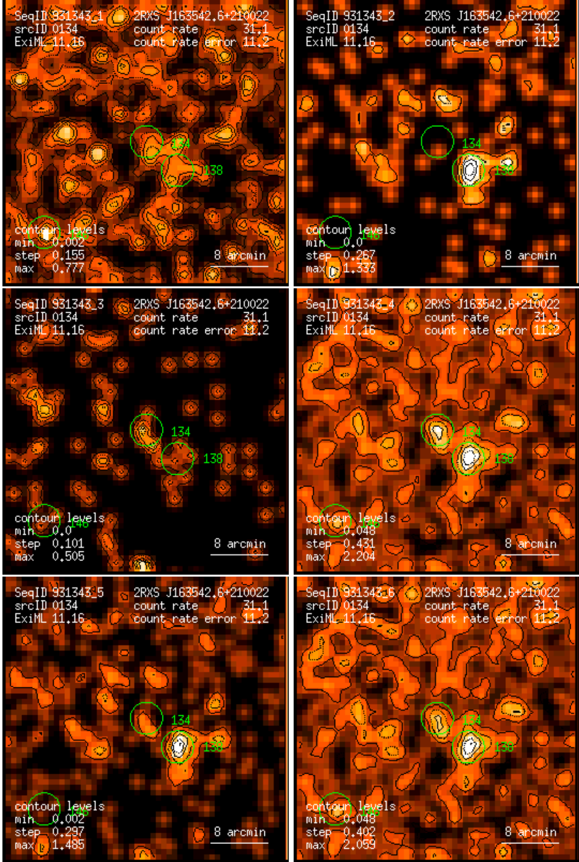
Figure 134: RASS 931343: detection 0134: band rate images, Gaussian filter: (1) PSPC channels 11 – 41, (2) 52 – 90, (3) 91 – 201, (4) 11 – 235, (5) 52 – 201, (6) 11 – 201. Broad band rates in counts/ks. Band rate contour levels in counts/ks/arcmin 2 .
