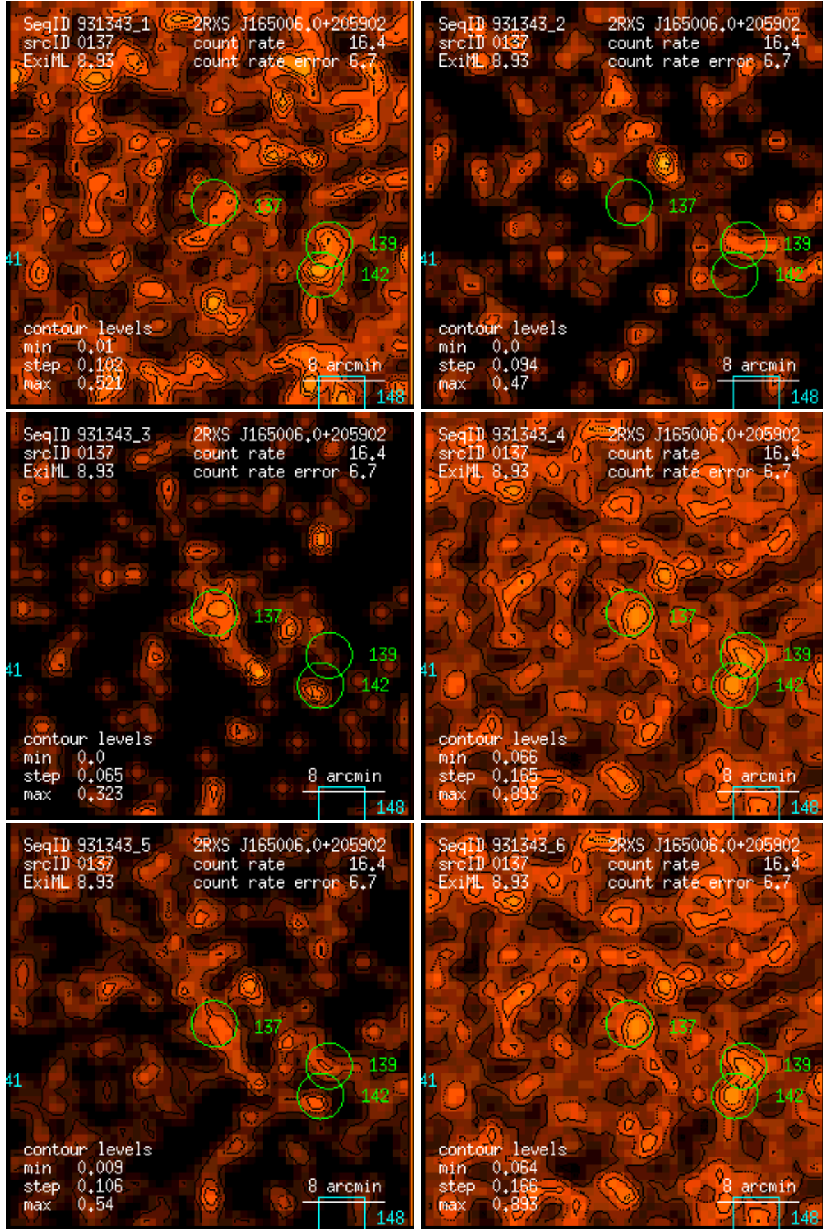
Figure 137: RASS 931343: detection 0137: band rate images, Gaussian filter: (1) PSPC channels 11 – 41, (2) 52 – 90, (3) 91 – 201, (4) 11 – 235, (5) 52 – 201, (6) 11 – 201. Broad band rates in counts/ks. Band rate contour levels in counts/ks/arcmin 2 .
